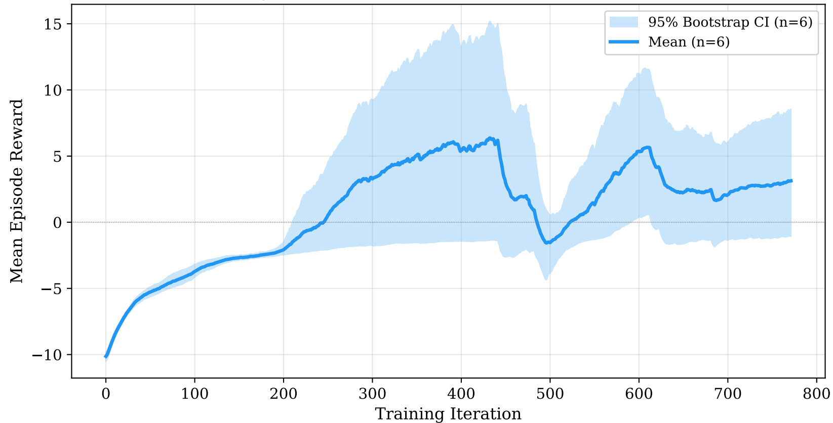
Training Reward: Mean with 95% Bootstrap CI (6 Seeds)
