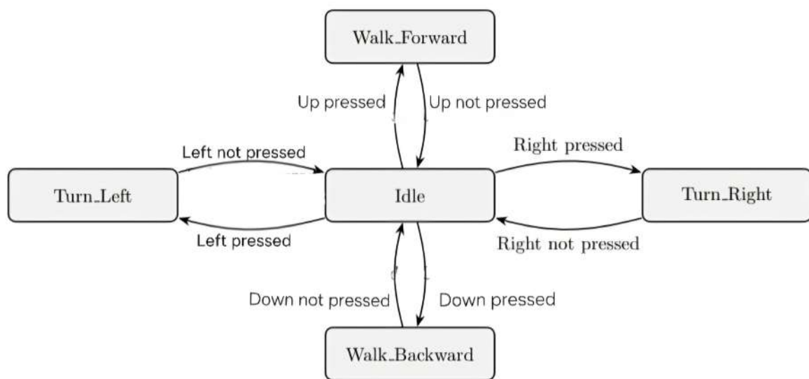
Figure 2: State Transition Diagram for Robot Movement
