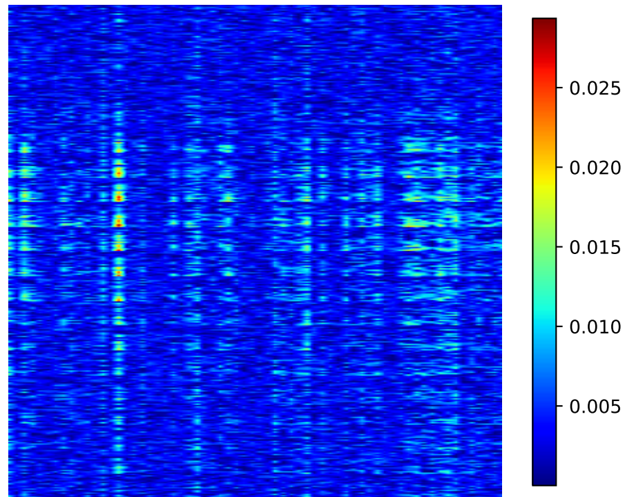
Grad-CAM Heatmap
