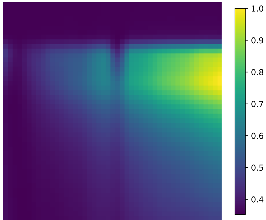
Grad-CAM Heatmap
