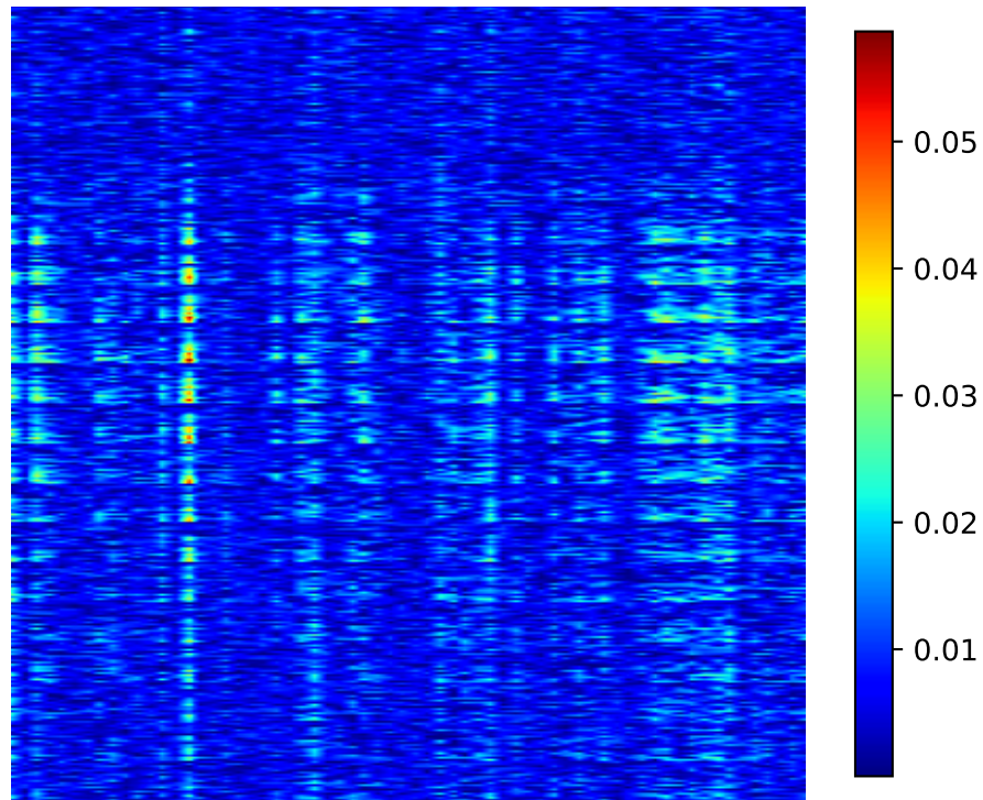
Grad-CAM Heatmap
