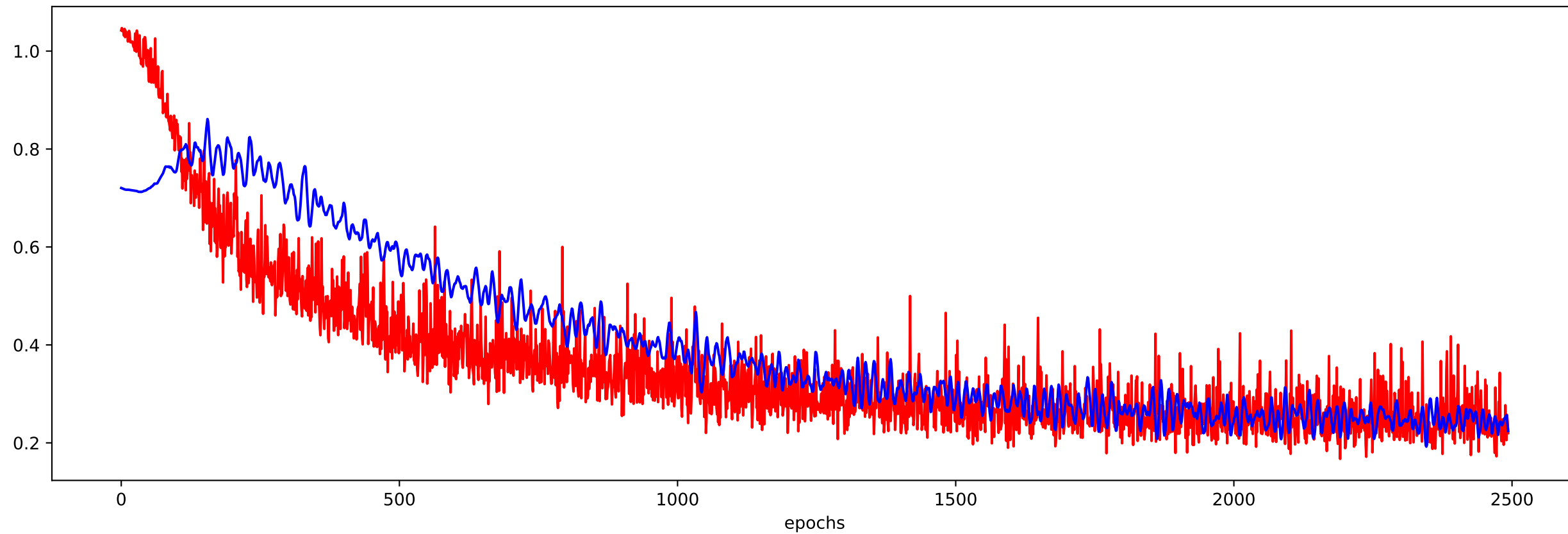
Model RMSE
