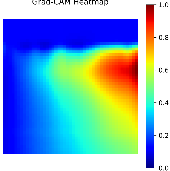
Grad-CAM Heatmap
