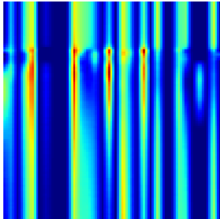
Grad-CAM Heatmap
