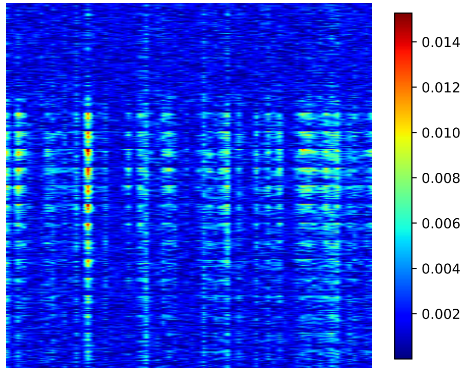
Grad-CAM Heatmap
