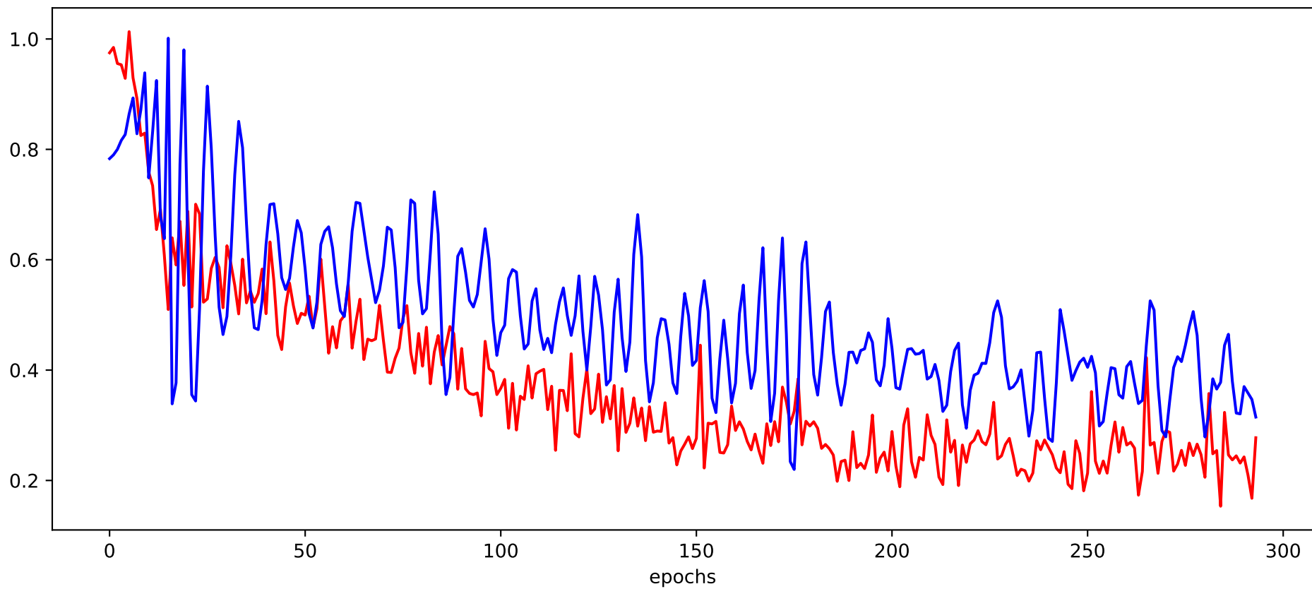
Model RMSE
