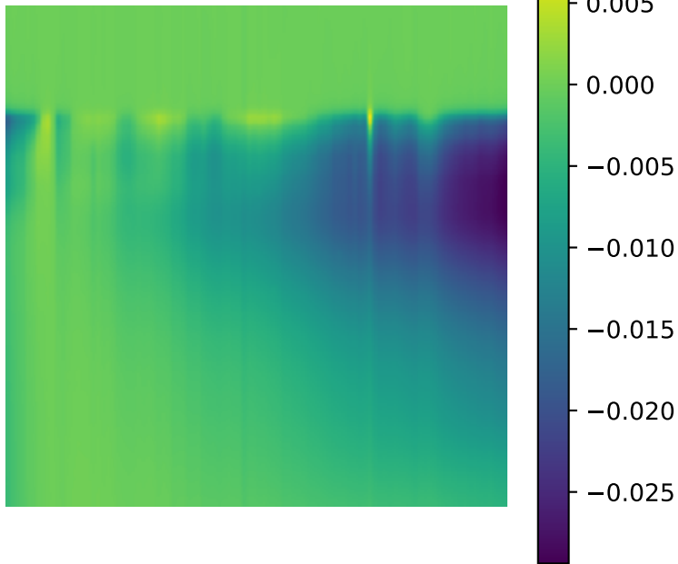
Qmatrix of the Cell 9
