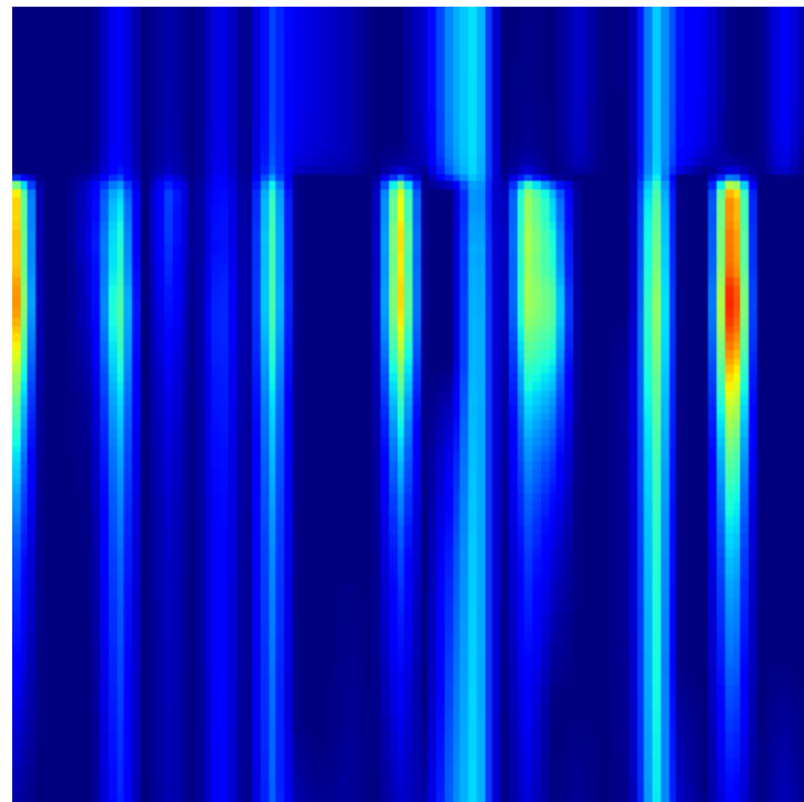
Grad-CAM Heatmap
