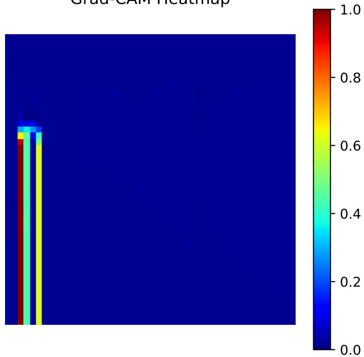
Grad-CAM Heatmap
