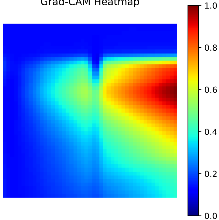
Grad-CAM Heatmap
