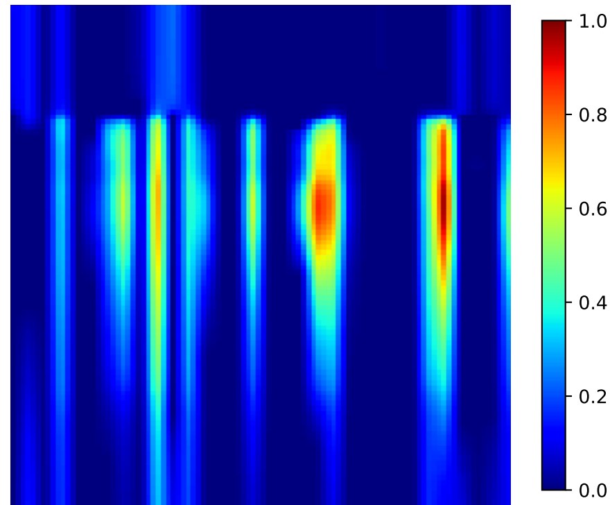
Grad-CAM Heatmap Best Model- 83.408
