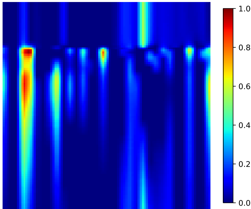
Grad-CAM Heatmap Worst Model- 40.396
