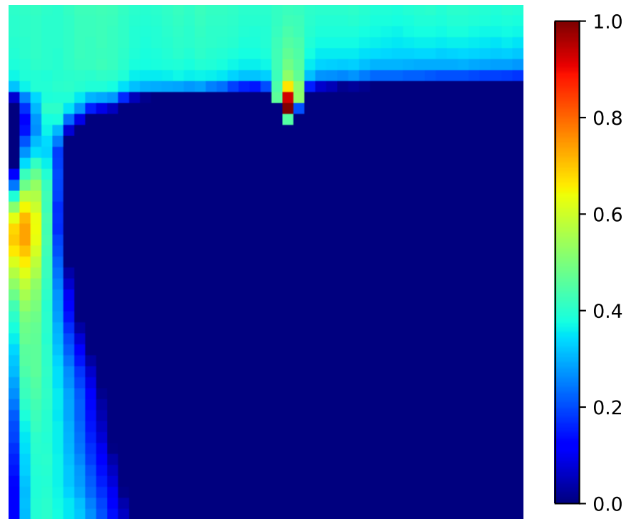
Grad-CAM Heatmap Worst Model- 38.376
