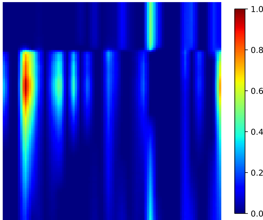
Grad-CAM Heatmap Worst Model- 62.841
