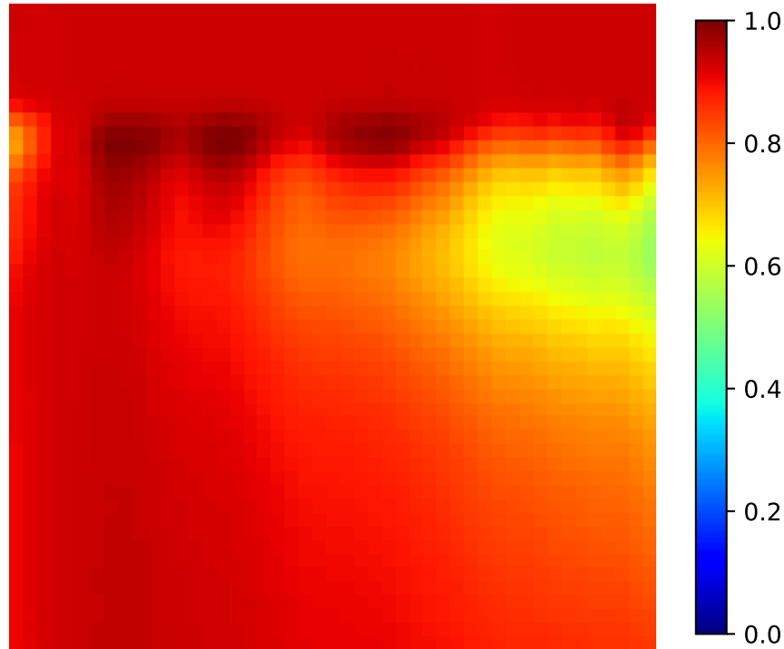
Grad-CAM Heatmap Worst Model- 27.765
