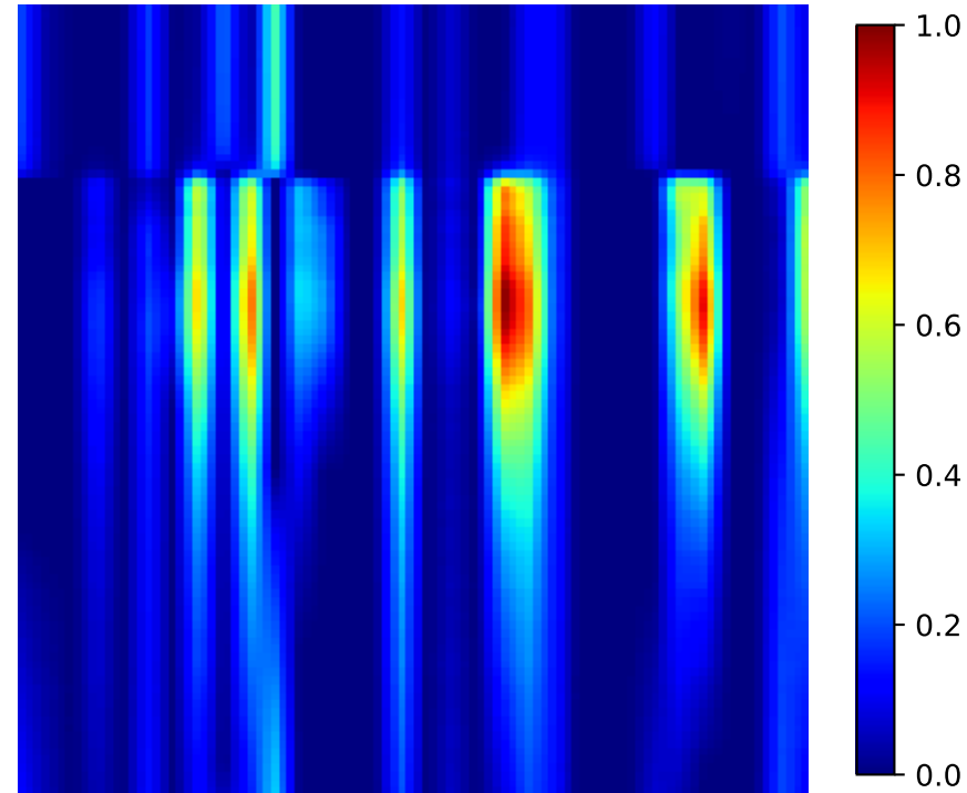
Grad-CAM Heatmap Best Model- 97.726
