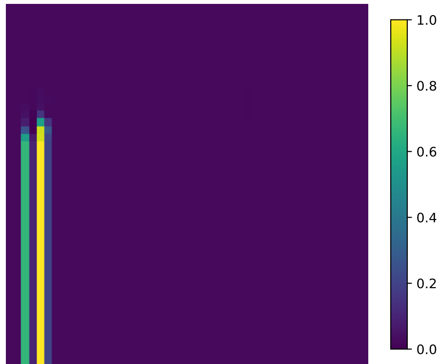
Grad-CAM Heatmap
