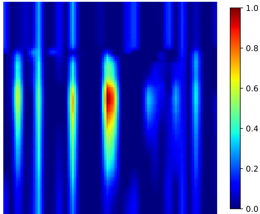
Grad-CAM Heatmap
