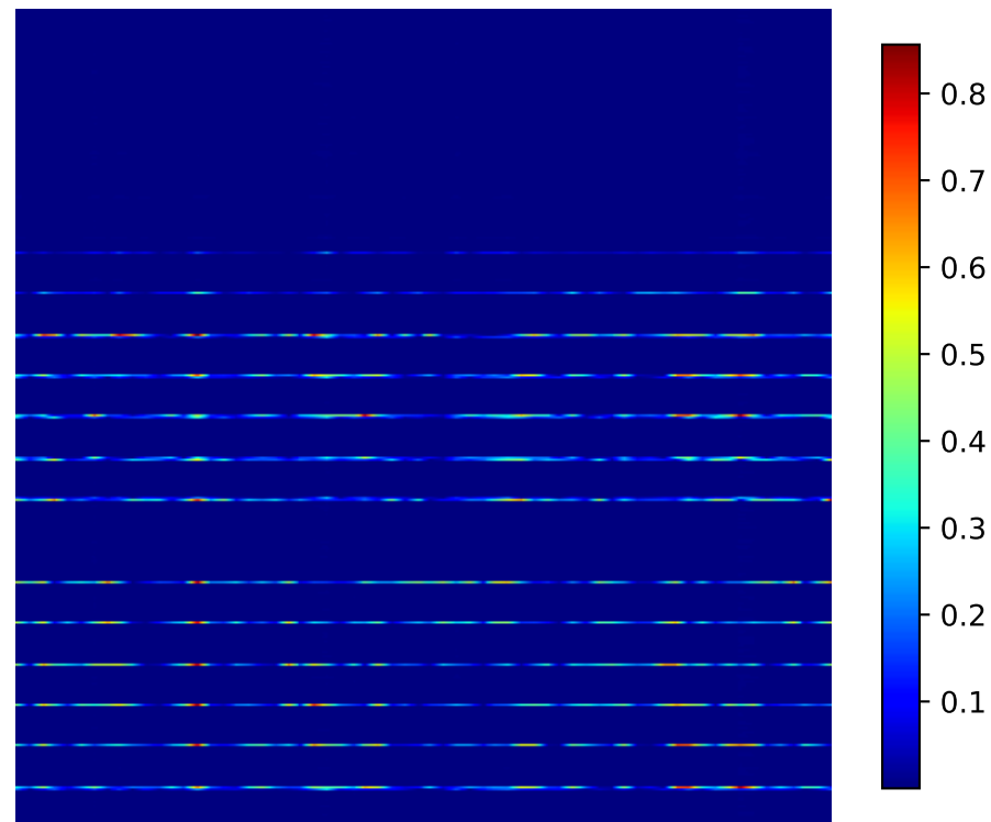
Grad-CAM Heatmap
