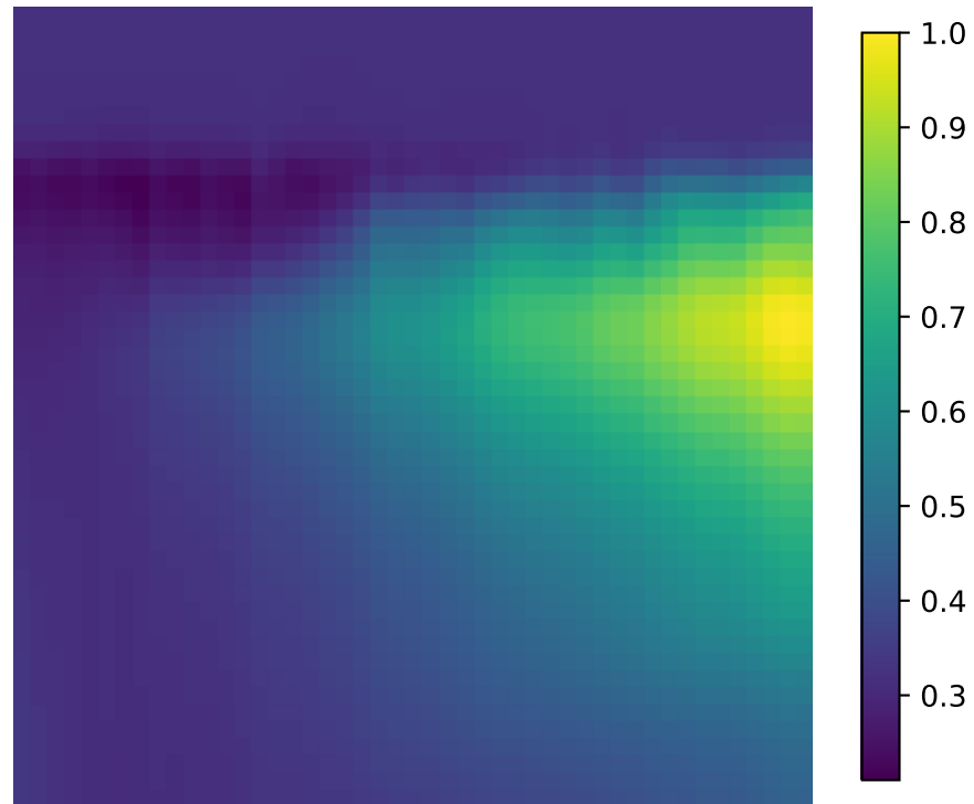
Grad-CAM Heatmap
