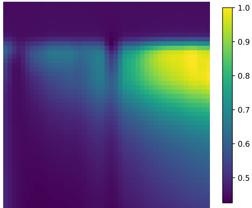
Grad-CAM Heatmap
