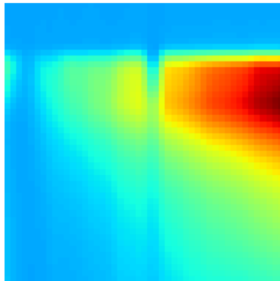
Grad-CAM Heatmap
