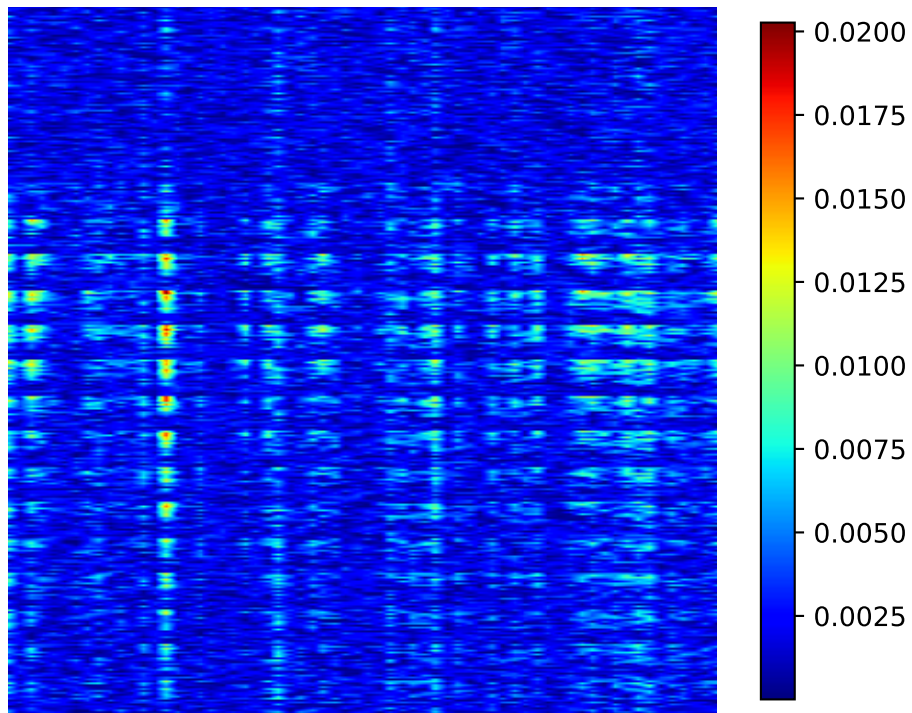
Grad-CAM Heatmap
