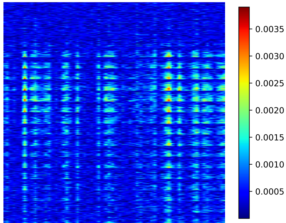
Grad-CAM Heatmap
