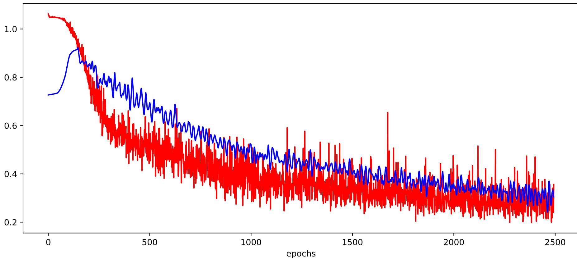
Model RMSE
