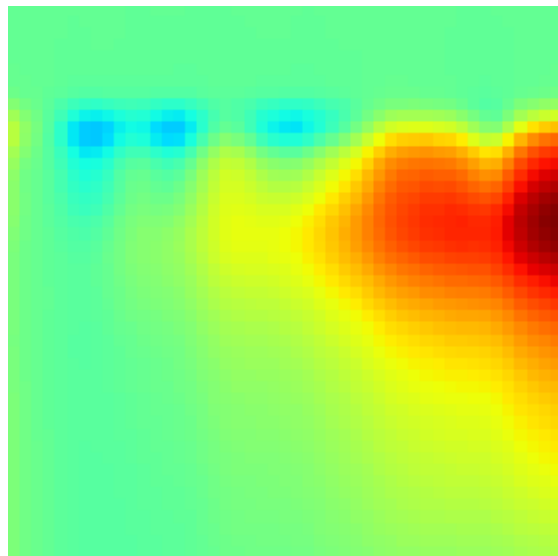
Grad-CAM Heatmap
