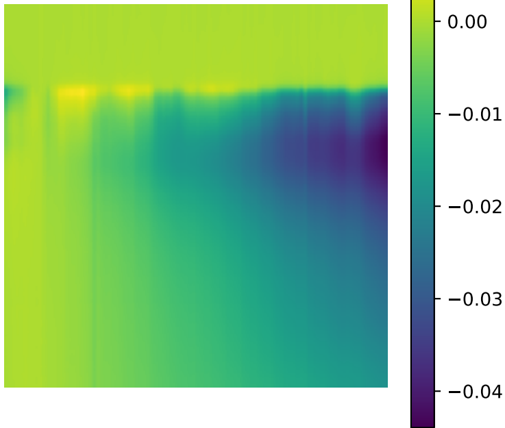
Qmatrix of the Cell 21
