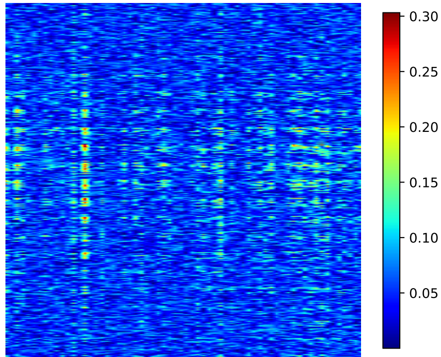
Grad-CAM Heatmap
