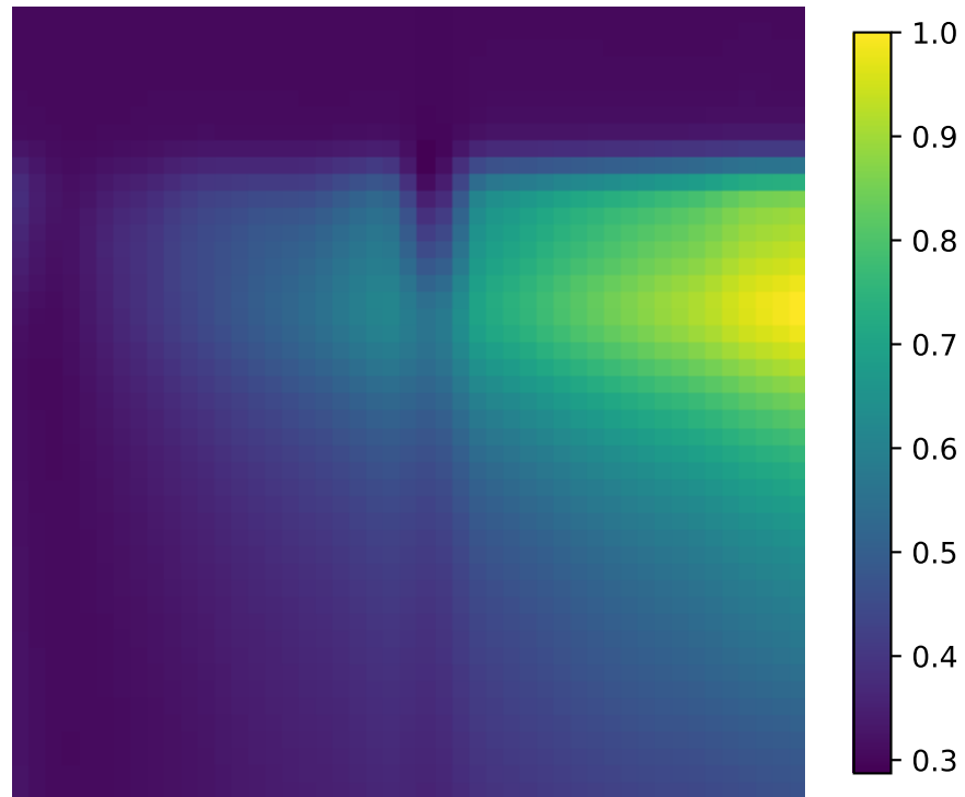
Grad-CAM Heatmap
