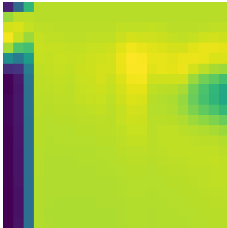
Grad-CAM Heatmap
