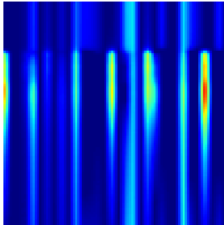
Grad-CAM Heatmap
