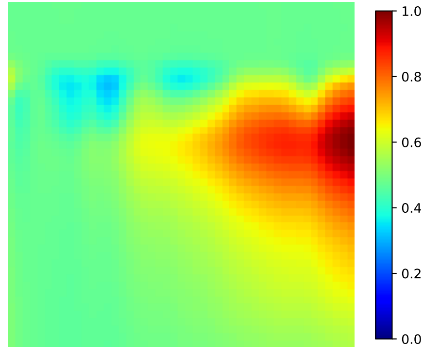
Grad-CAM Heatmap Best Model- 95.220
