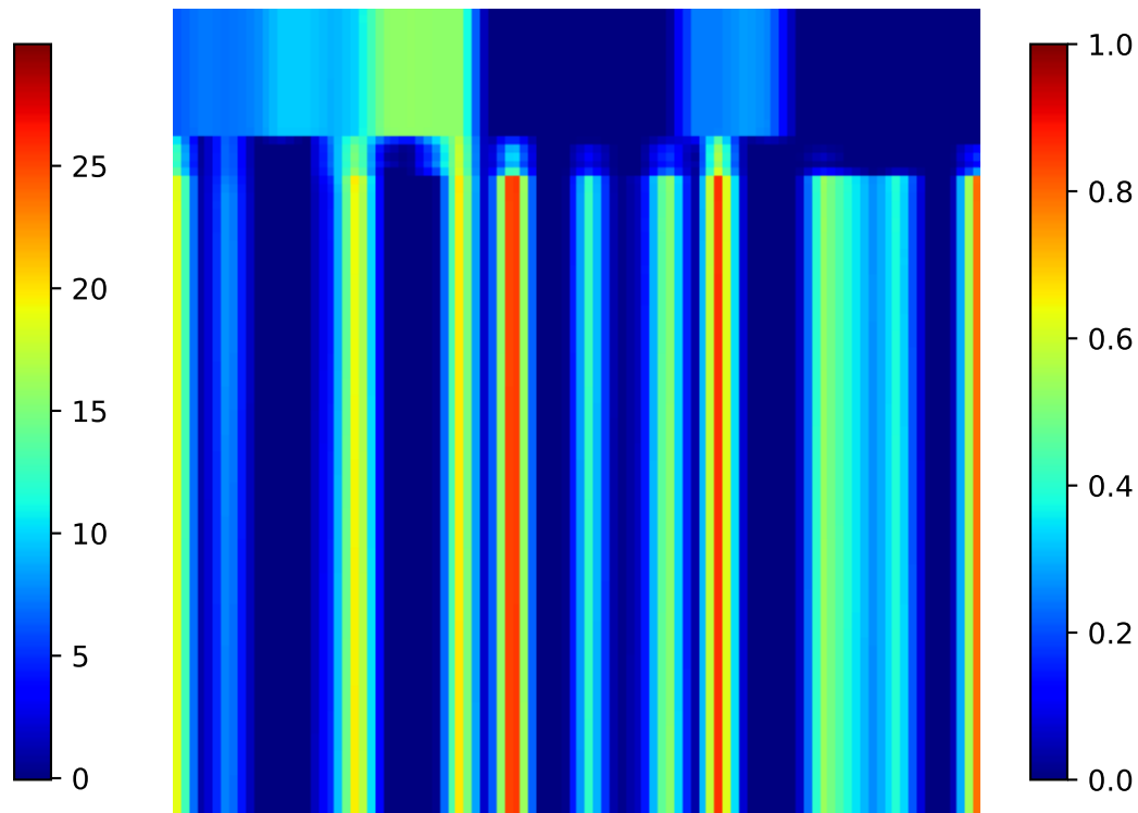
Grad-CAM Heatmap
