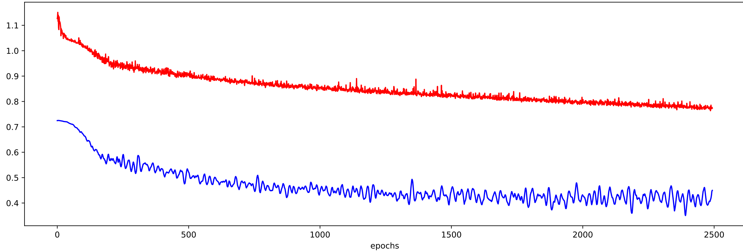
Model RMSE
