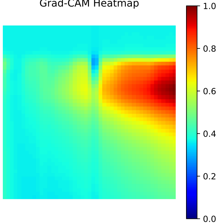
Grad-CAM Heatmap
