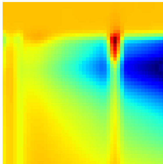
Grad-CAM Heatmap
