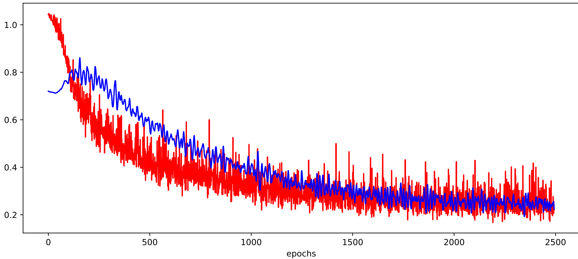
Model RMSE
