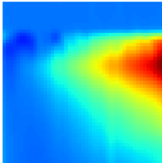
Grad-CAM Heatmap
