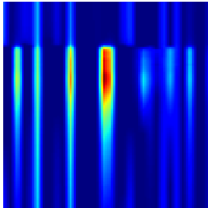
Grad-CAM Heatmap
