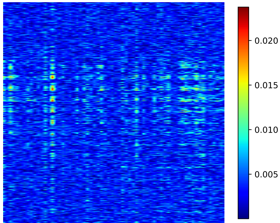
Grad-CAM Heatmap
