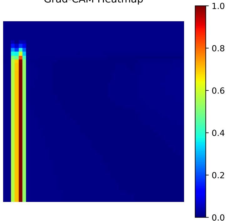
Grad-CAM Heatmap
