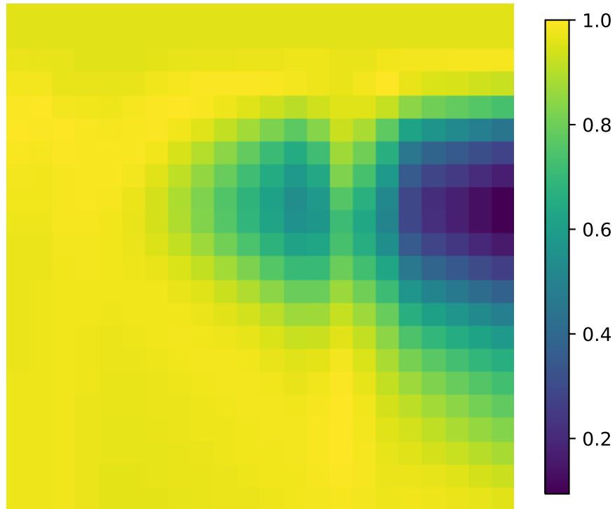
Grad-CAM Heatmap
