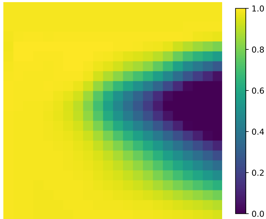
Grad-CAM Heatmap
