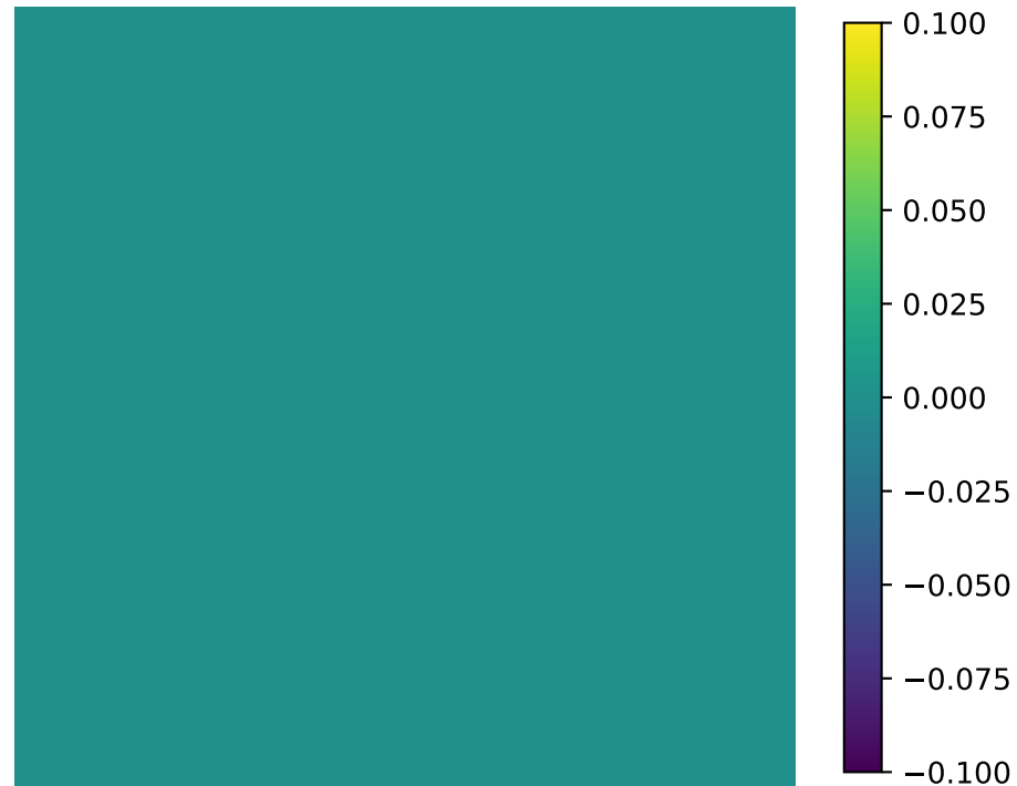
Grad-CAM Heatmap
