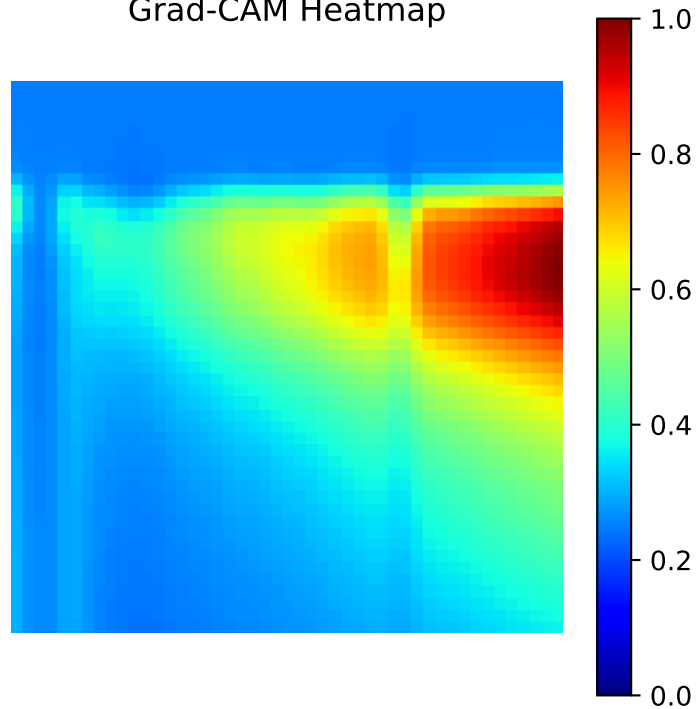
Grad-CAM Heatmap
