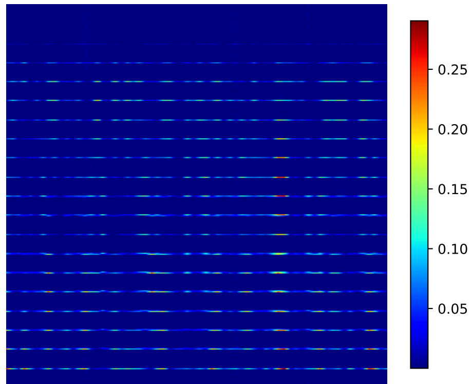
Grad-CAM Heatmap
