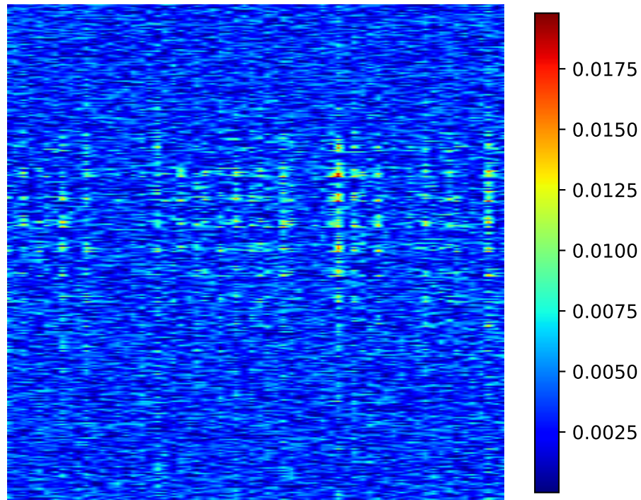
Grad-CAM Heatmap
