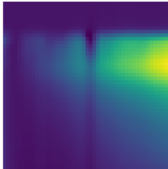
Grad-CAM Heatmap
