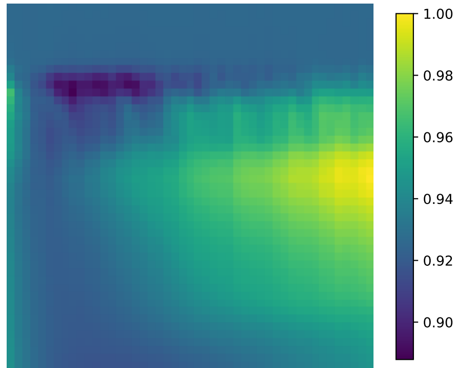
Grad-CAM Heatmap
