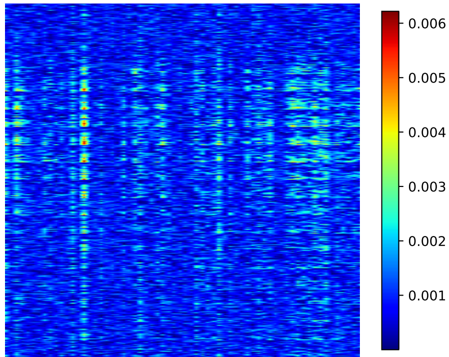
Grad-CAM Heatmap
