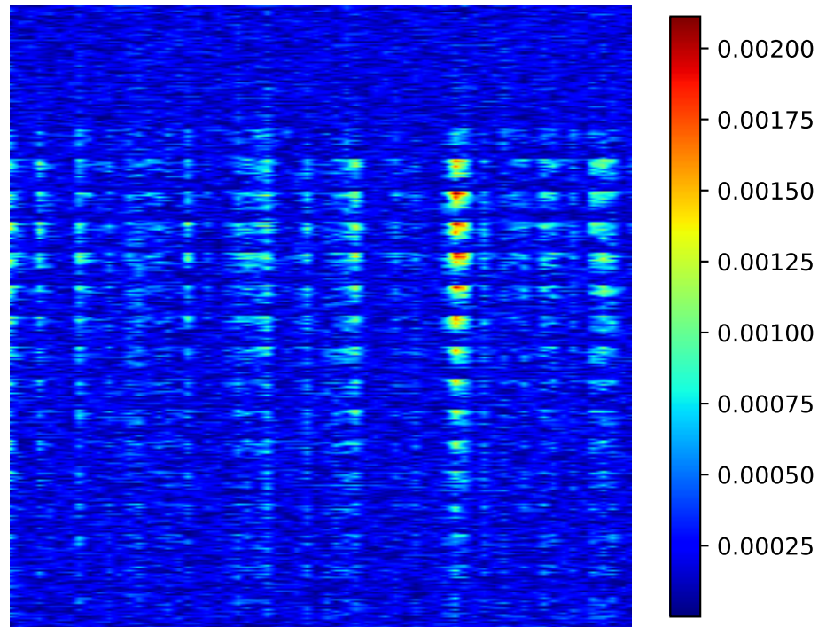
Grad-CAM Heatmap
