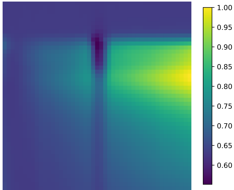
Grad-CAM Heatmap
