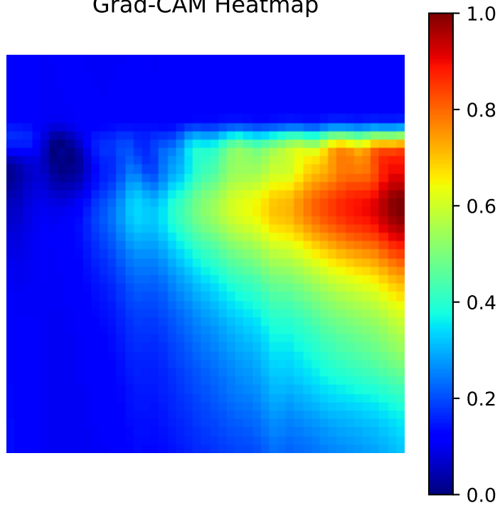
Grad-CAM Heatmap
