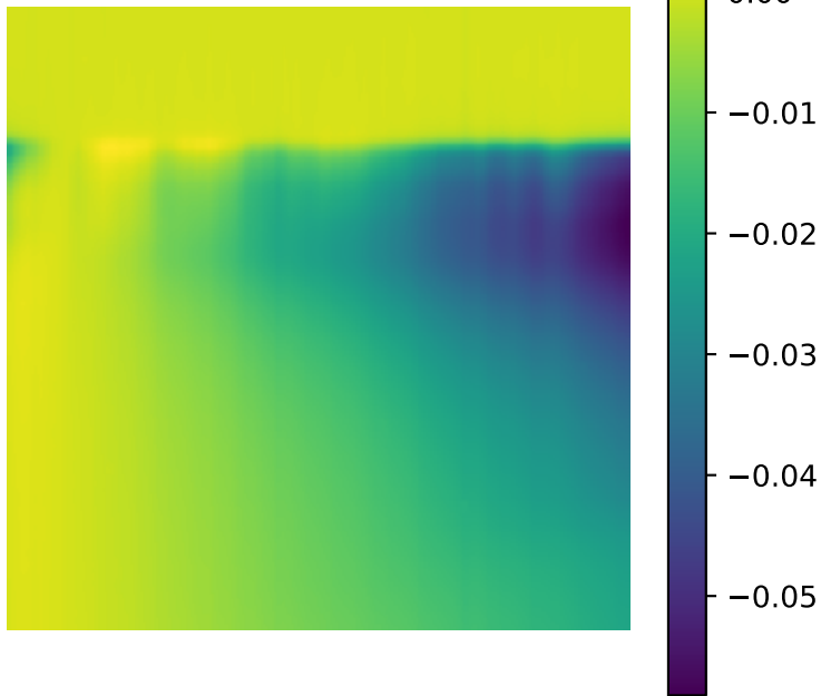
Qmatrix of the Cell 27
