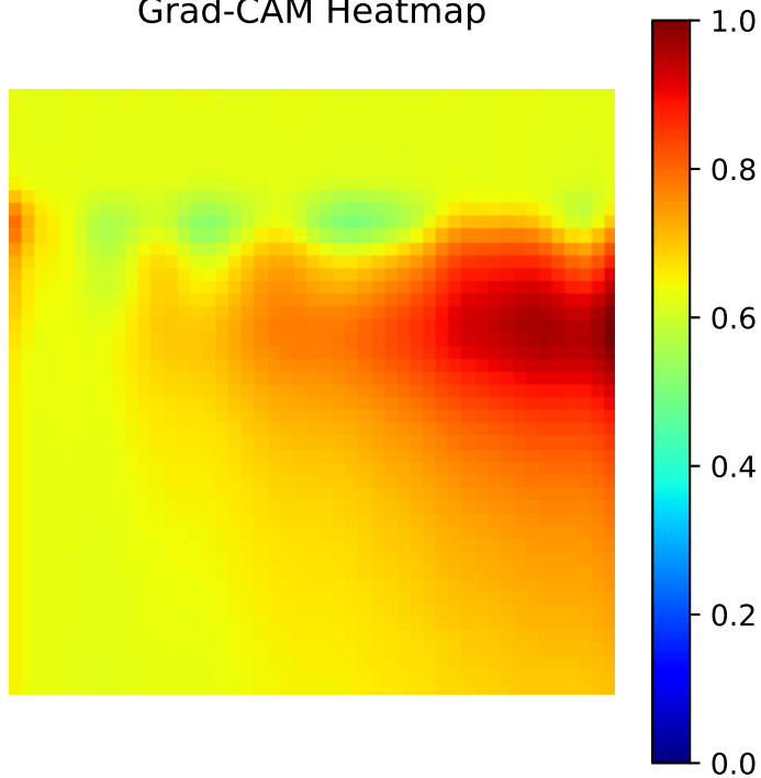
Grad-CAM Heatmap
