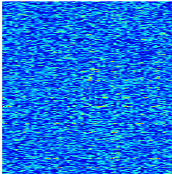
Grad-CAM Heatmap
