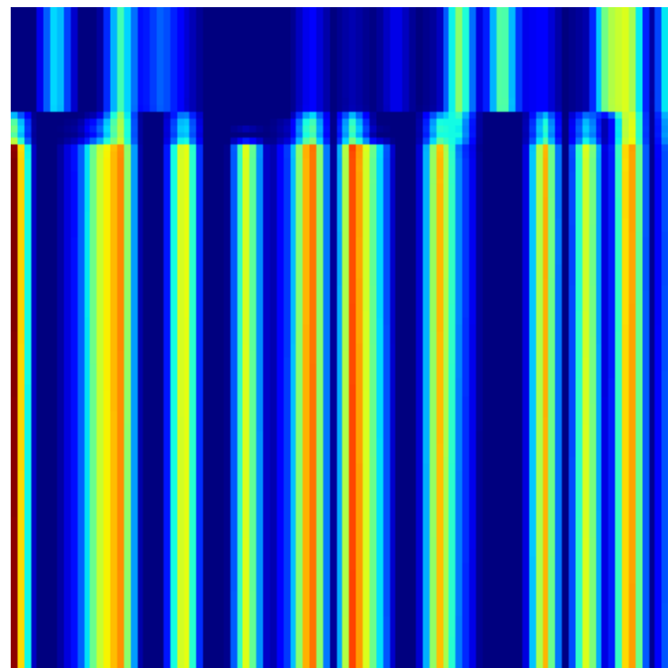
Grad-CAM Heatmap
