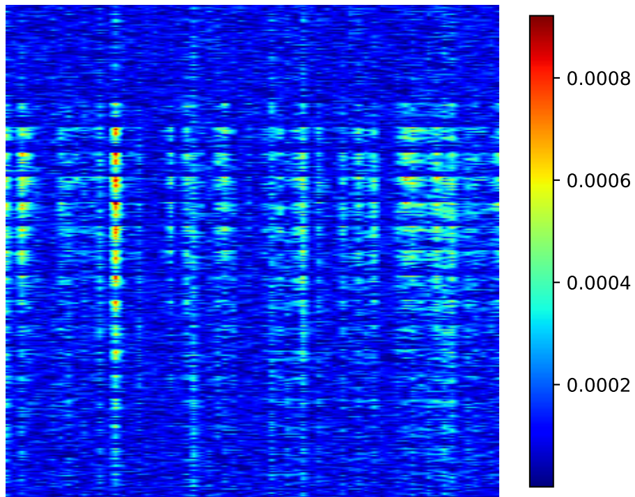
Grad-CAM Heatmap
