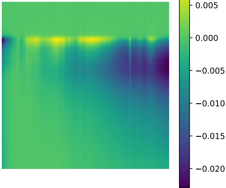
Qmatrix of the Cell 2
