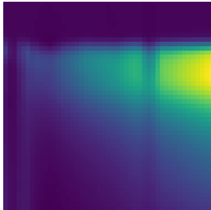
Grad-CAM Heatmap
