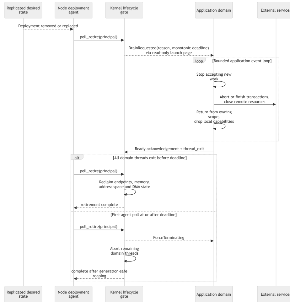
Figure 17.5: Bounded cooperative shutdown followed by generation-safe forced retirement. The application can acknowledge but cannot clear or extend a kernel-published lifecycle request.
