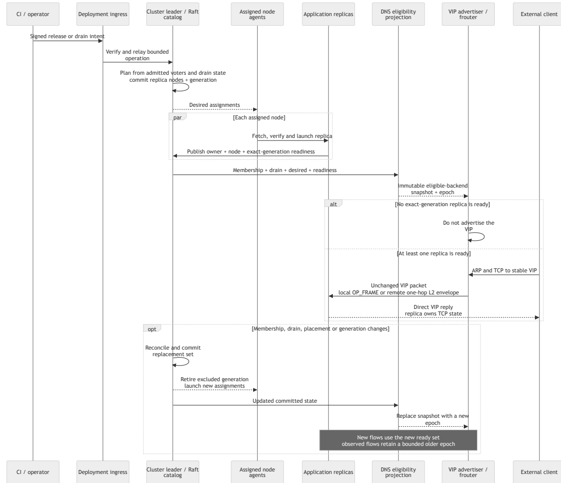
Figure 13.1: Cluster management supplies DSR with an exact-generation eligible-backend set; packet steering remains outside the consensus path.
