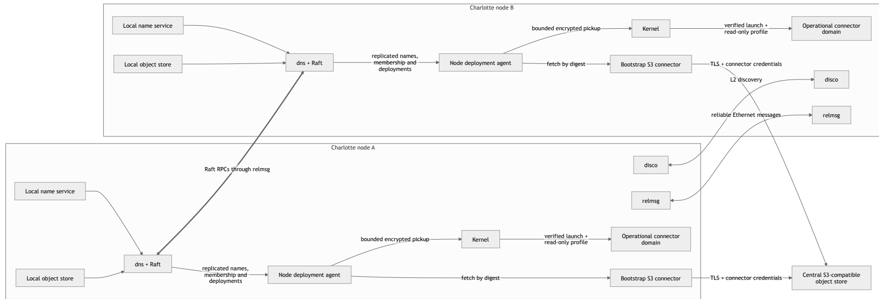
Figure 17.4: A focused two-guest deployment fixture combines Raft-held desired state, local reconcilers, capability-routed services, and central object pickup; the architecture admits larger voter and replica sets.
