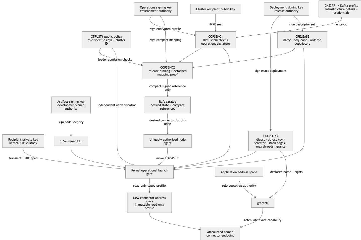
Figure 17.5: Independent artifact, deployment, operations, and recipient-key roles converge only at cluster admission and the privileged connector launch gate.
