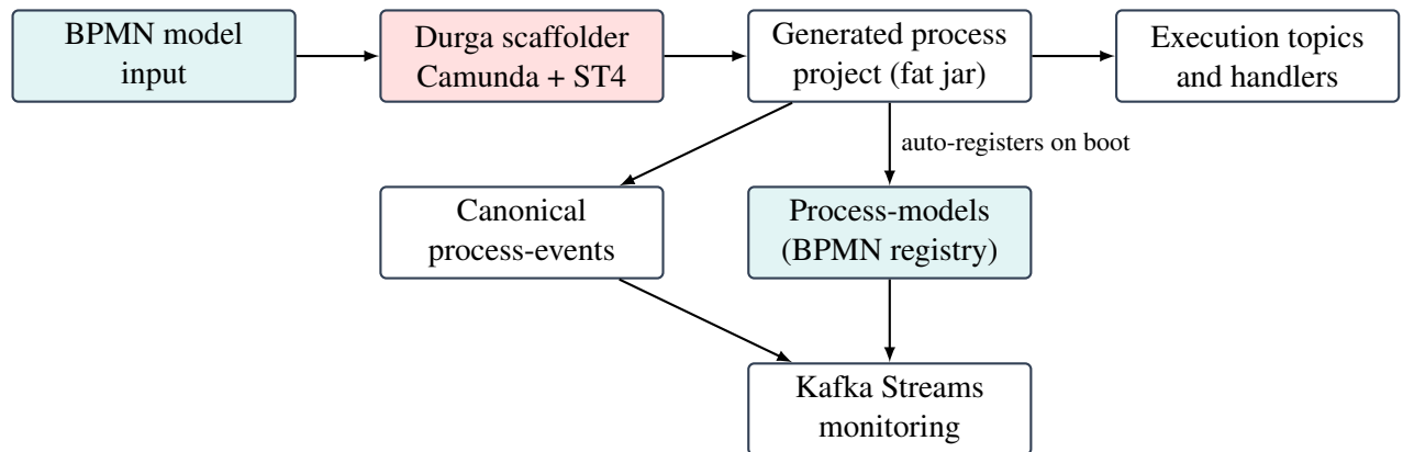
Figure 1: High-level flow: BPMN model → generated runtime → self-registration → monitoring
