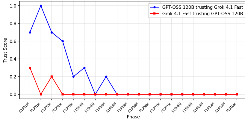
Figure 4: Asymmetric trust dynamics: Grok 4.1 Fast’s trust drops to 0.0 by F1901M while GPT-OSS 120B maintains high trust, unaware of the betrayal.
