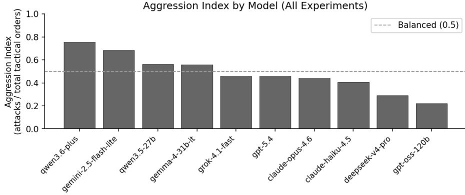
Figure 3: Aggression index by model (ratio of attack orders to total tactical orders). Higher values indicate more offensive play.
