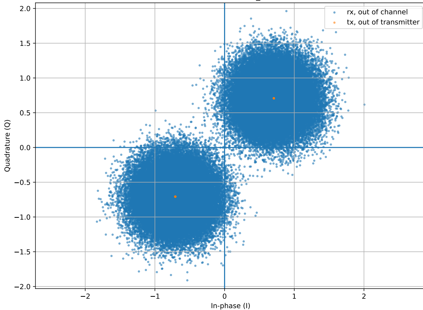
Constellation for SNR_dB=8.0
