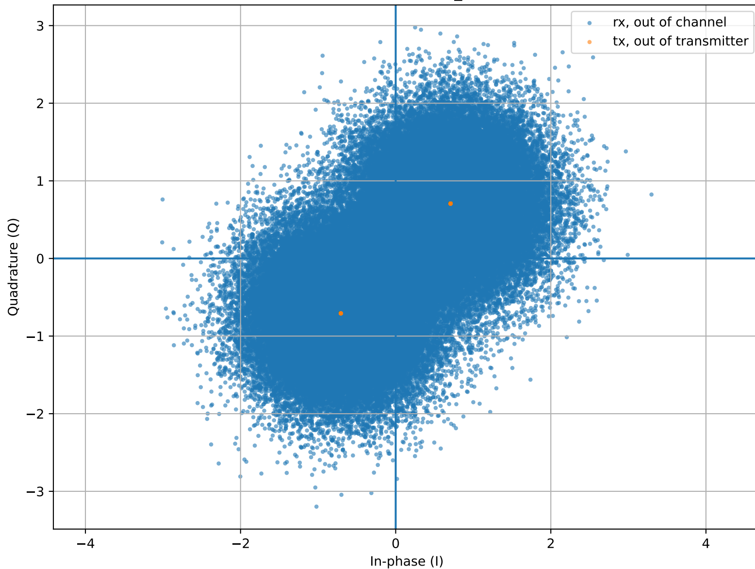
Constellation for SNR_dB=2.0
