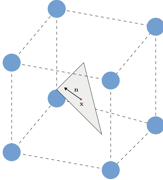
Figure 7: Illustration of a surface query. The surface point \mathbf{x} is used to locate the eight nearest probes making up the surrounding probe cage. Then, the surface normal \mathbf{n} is used as the sampling direction to query each probe’s irradiance cache.
