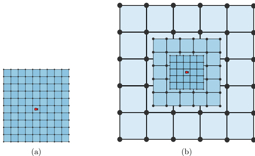
Figure 3: Comparison between a 2D top-view of a uniform and cascaded probe volume using the same probe budget (the same ideas also apply to the third dimension). The left image shows a 10 \times 11 uniform grid for a total of 110 probes, while the right image shows a 3-level cascaded grid for a total of 108 probes (36 per cascade). The spatial resolution of the uniform grid and cascade c = 0 are equivalent, showing how the cascaded version allows for a larger scene coverage while using the same number of probes.
