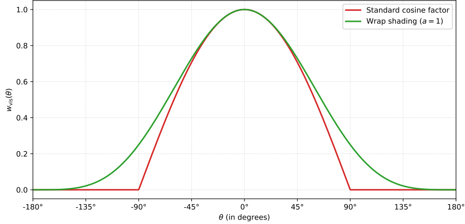
Figure 10: Comparison between two different visibility attenuation functions. The red curve shows the standard Lambertian cosine factor while the green curve illustrates the wrap shading function as implemented in DDGI [29]. Notice their behaviors at grazing angles: while wrap shading smoothly decreases light contribution, the standard cosine factor results in an abrupt cut instead.
