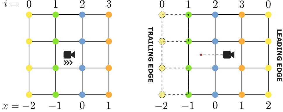
Figure 4: Top-down view of a single probe volume cascade (i.e., with constant, unit probe spacing), as each cascade is moved independently of the others. As the camera moves one cell to the right, the cascade origin snaps by its probe spacing, keeping existing probes stationary while trailing edge probes are recycled to cover the newly exposed leading edge. Under toroidal addressing (Equation 3.2), tile index i_x = 0 and its corresponding memory slot are recycled without disturbing the remaining green, blue, and orange probes.
