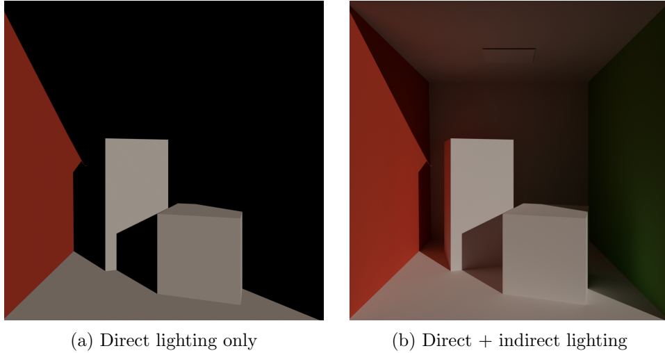
Figure 2: Render of the Cornell Box scene using Blender’s Cycles, illuminated by a single light source simulating the Sun. The left image (a) displays direct illumination only while the right image (b) includes both the direct and indirect components, resulting in a more realistic look. Also notice how the red color from the left wall bleeds onto the white box.
