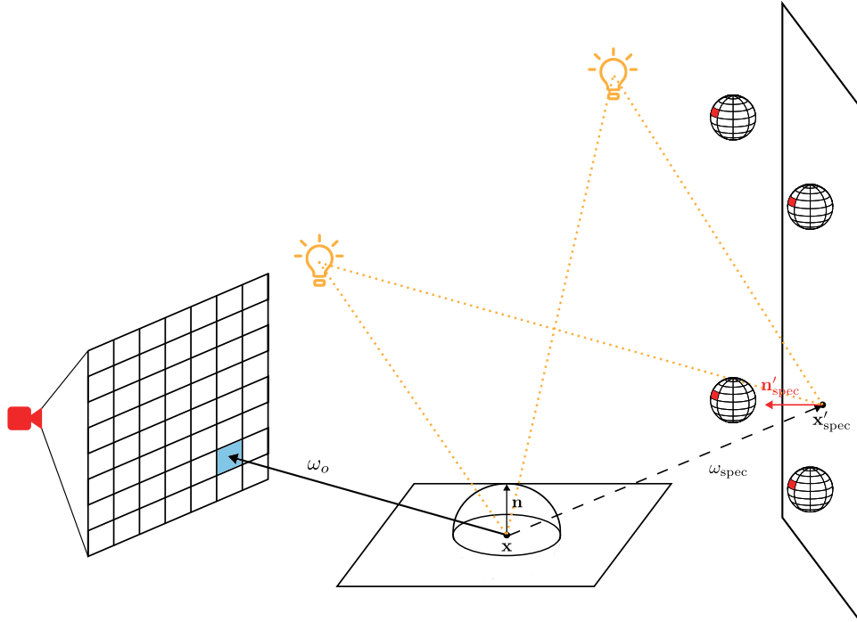
Figure 12: Schematic representation of all the elements involved in the shading of surface point \mathbf{x} . Here, to evaluate the indirect specular illumination, a ray is cast along the importance-sampled direction \omega_{\text{spec}} . Apart from the choice of sampling direction, the overall evaluation procedure mirrors that of the diffuse pass.
