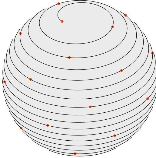
Figure 9: A SF sequence of 30 sample points are generated over the unit sphere following Equation 4.1. These sample points are then used to compute the set of directions toward which the rays are cast.
