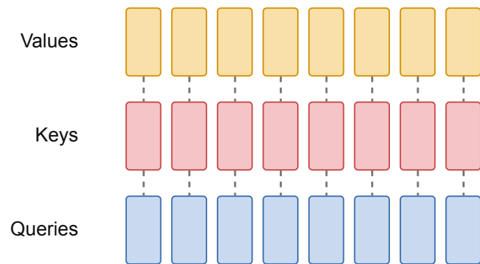
Multi-Head Attention
