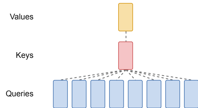
Multi-Query Attention
