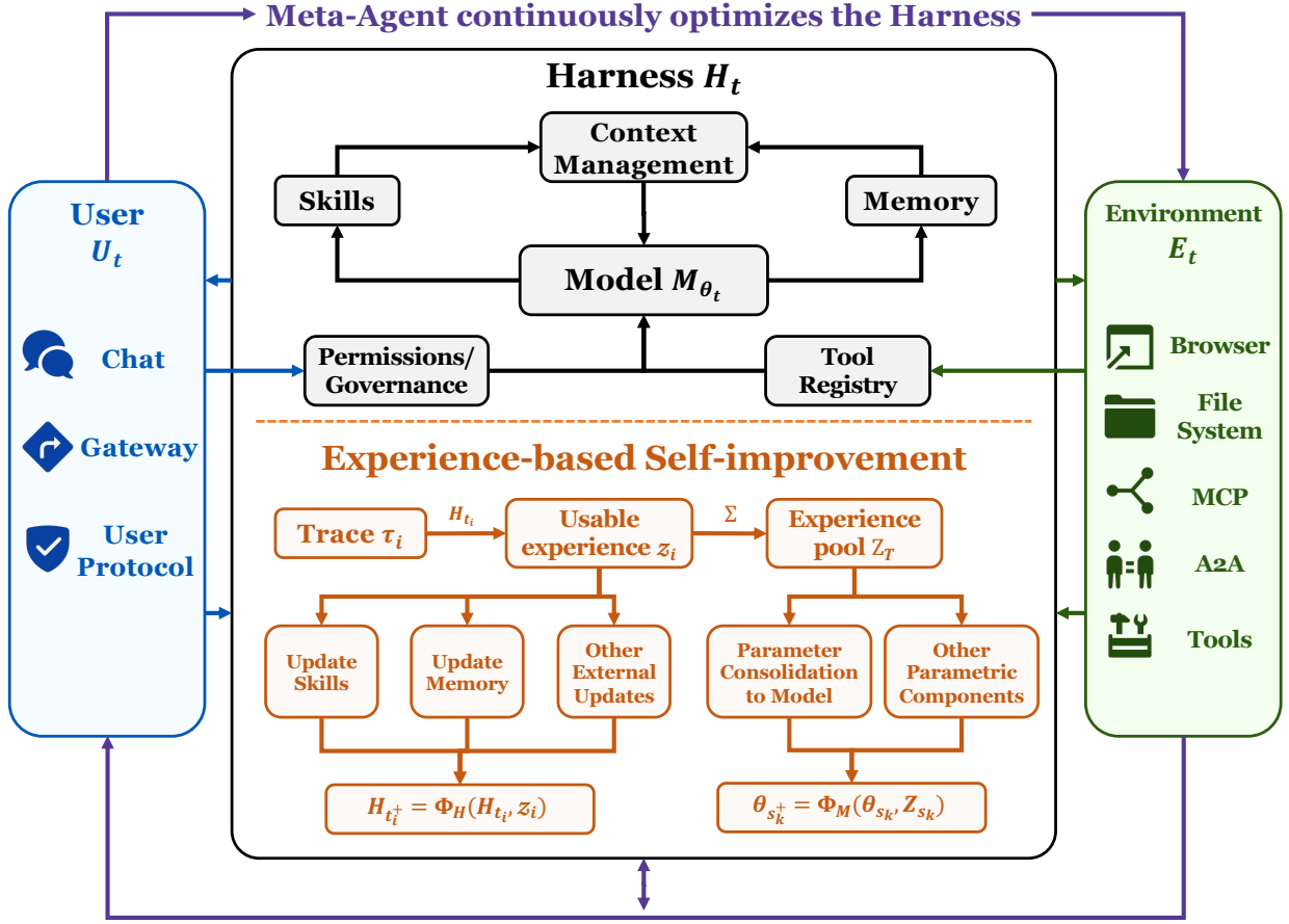
Figure 2 | Harness as experience infrastructure for deployed agents. The user side U_t supplies goals, instructions, preferences, approvals, and corrections, while the environment side E_t supplies executable state, observations, tests, and verifiable feedback. The harness H_t mediates context, action routing, permissions, and trace compilation, turning interaction traces into usable experience that can update skills, memory, other external components, or model parameters.
