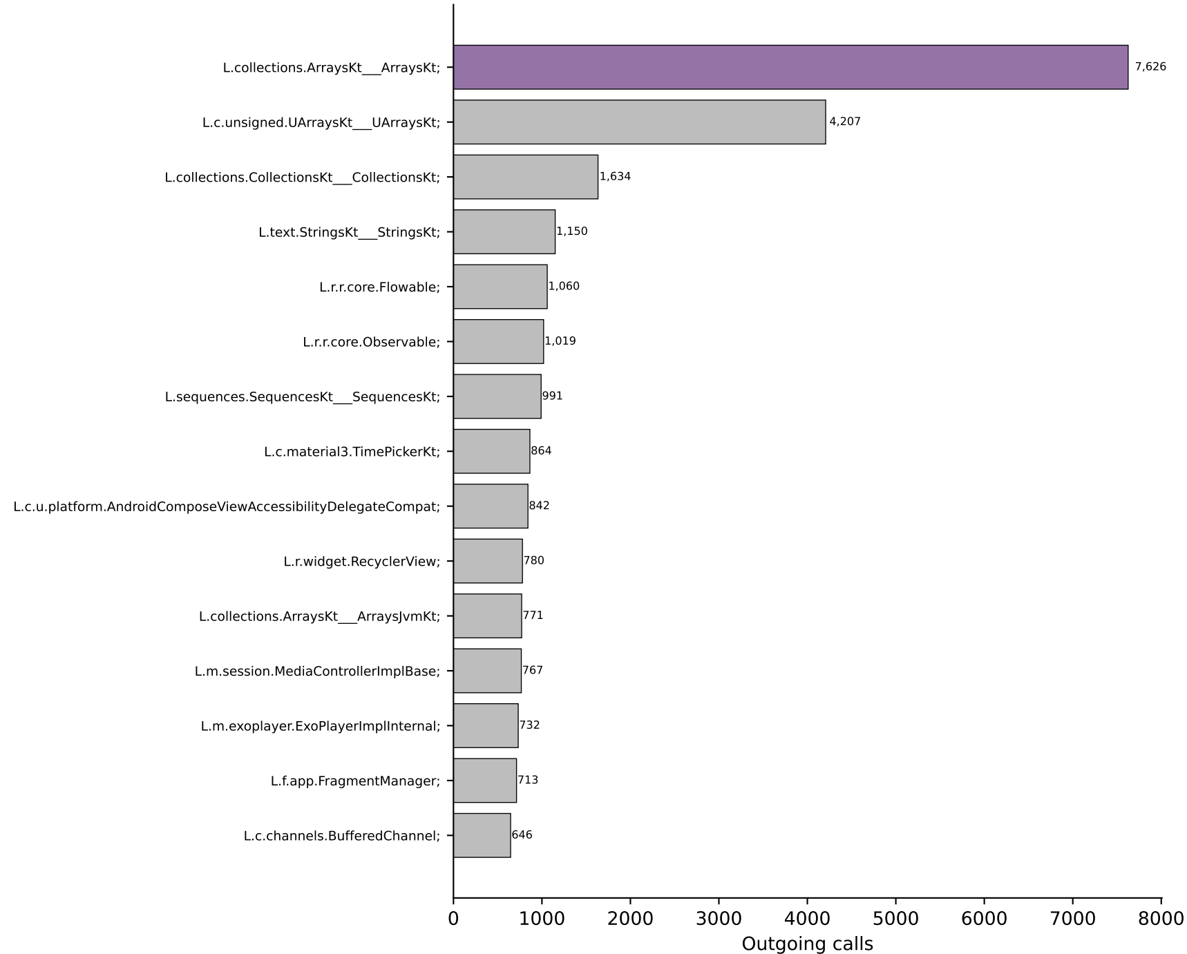
Top 15 Callers
