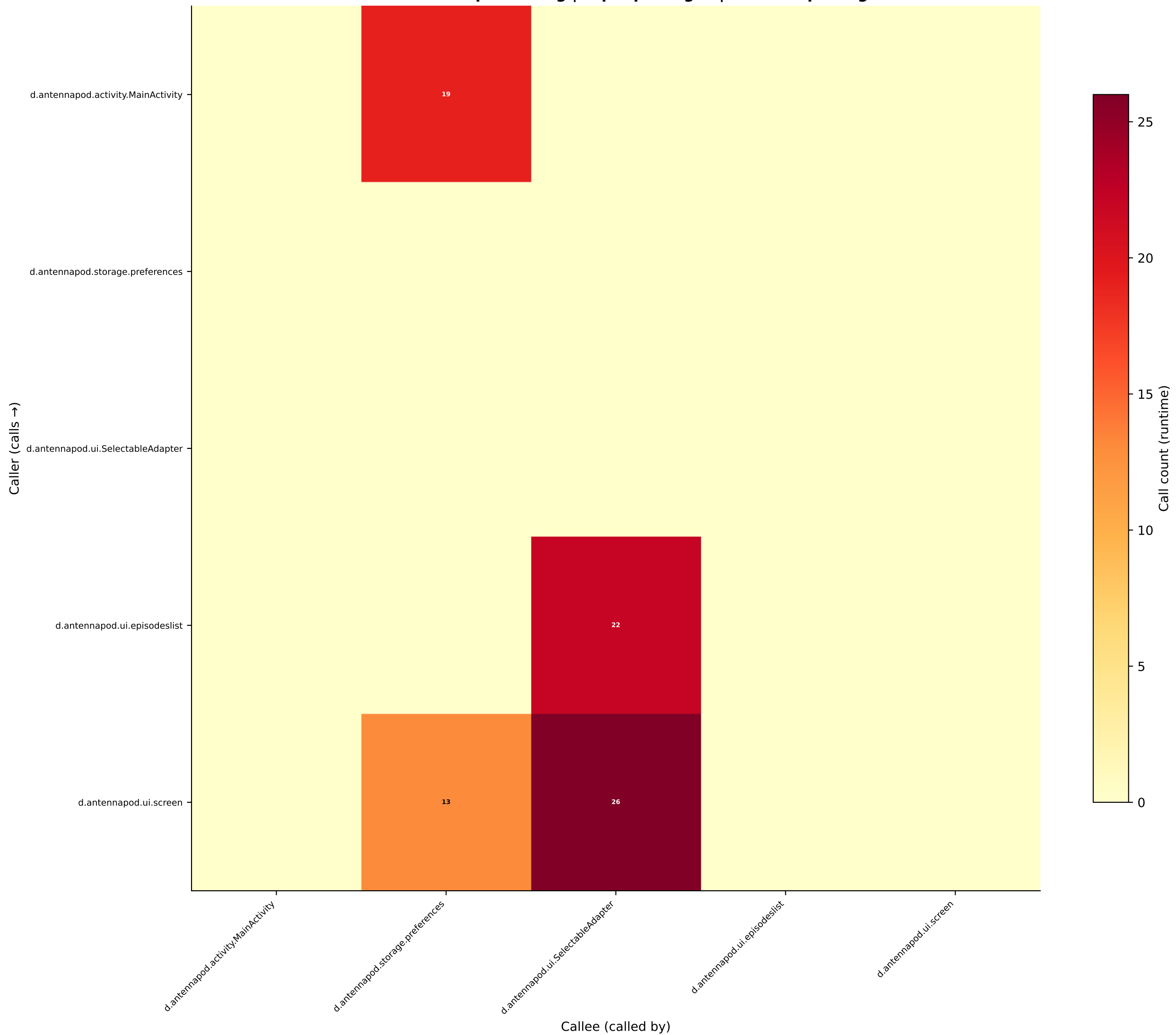
Package Interaction Heatmap — Frida Runtime Trace de.danoeh.antennapod.debug | Top 5 packages | 80 cross-package calls
