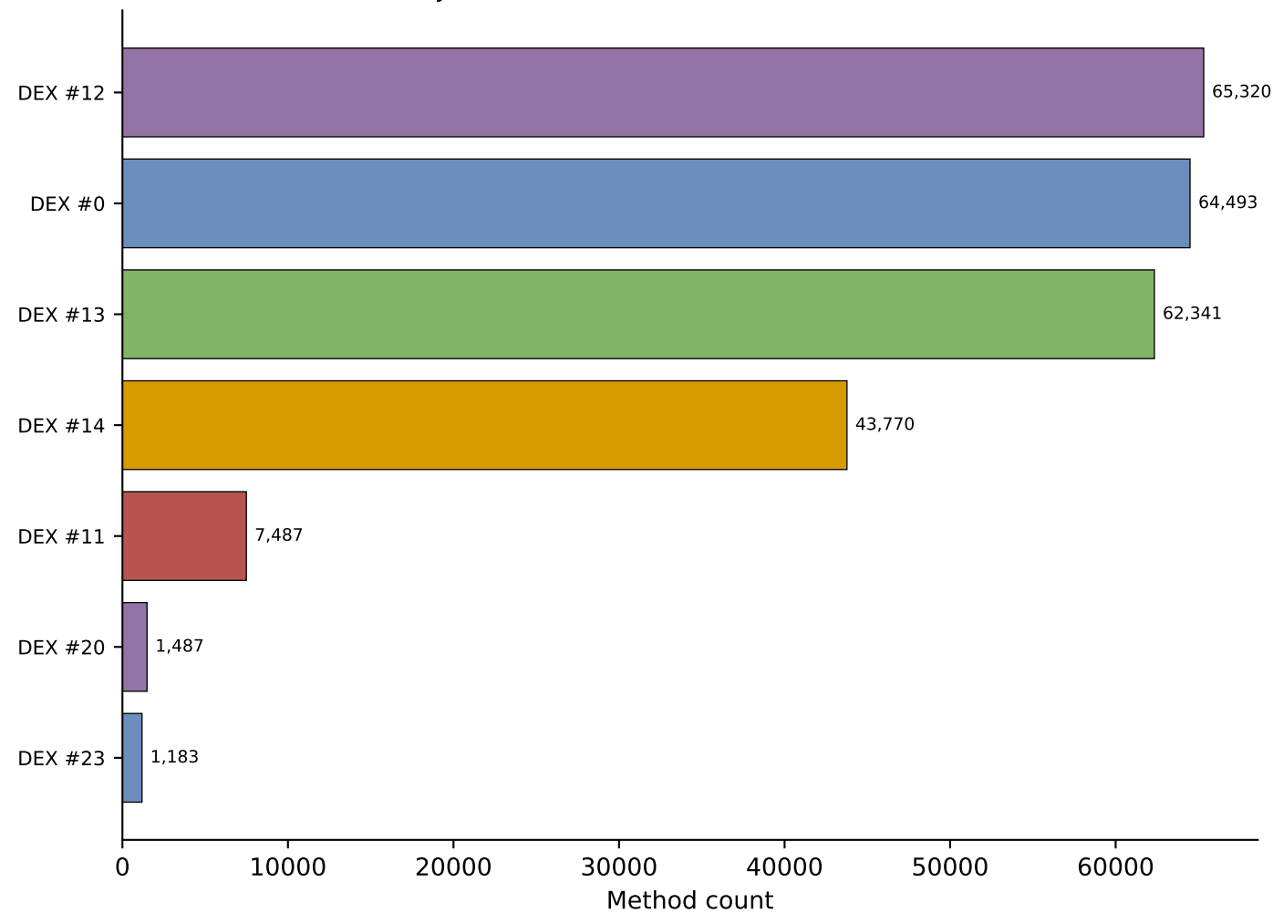
Major DEX Files (7 with >1000 methods)
