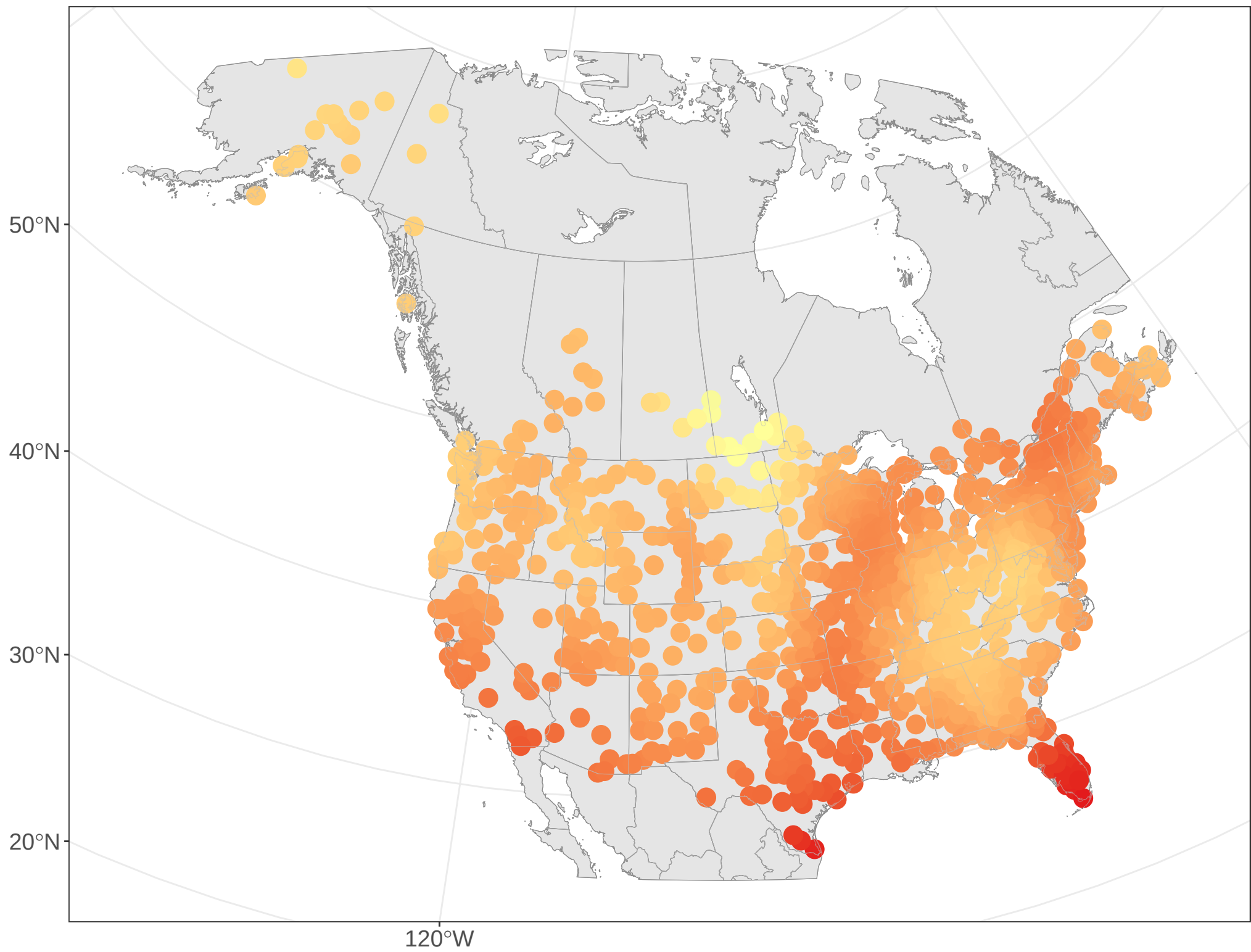
ab_trend_gam
