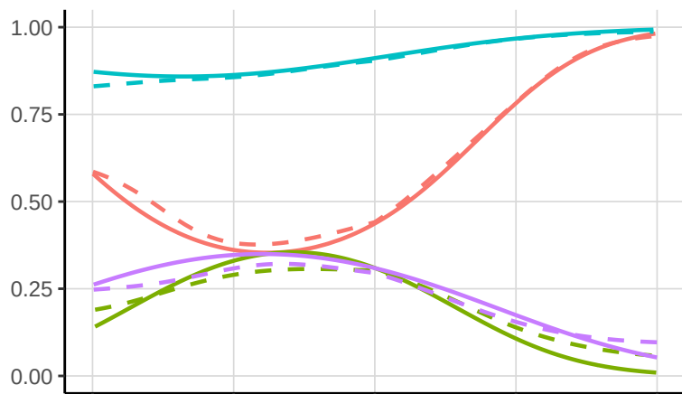
\phi (survival)
