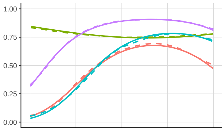
p (detection)
