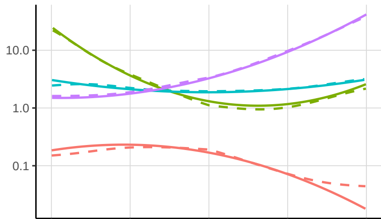
\gamma (recruitment)
