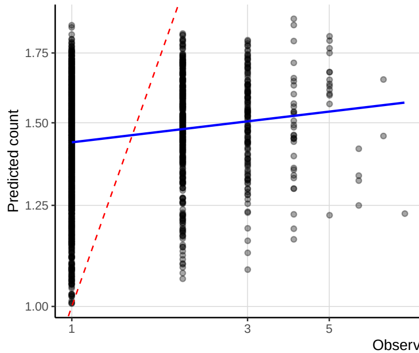
Bayesian
