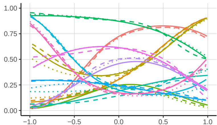
\phi (survival)
