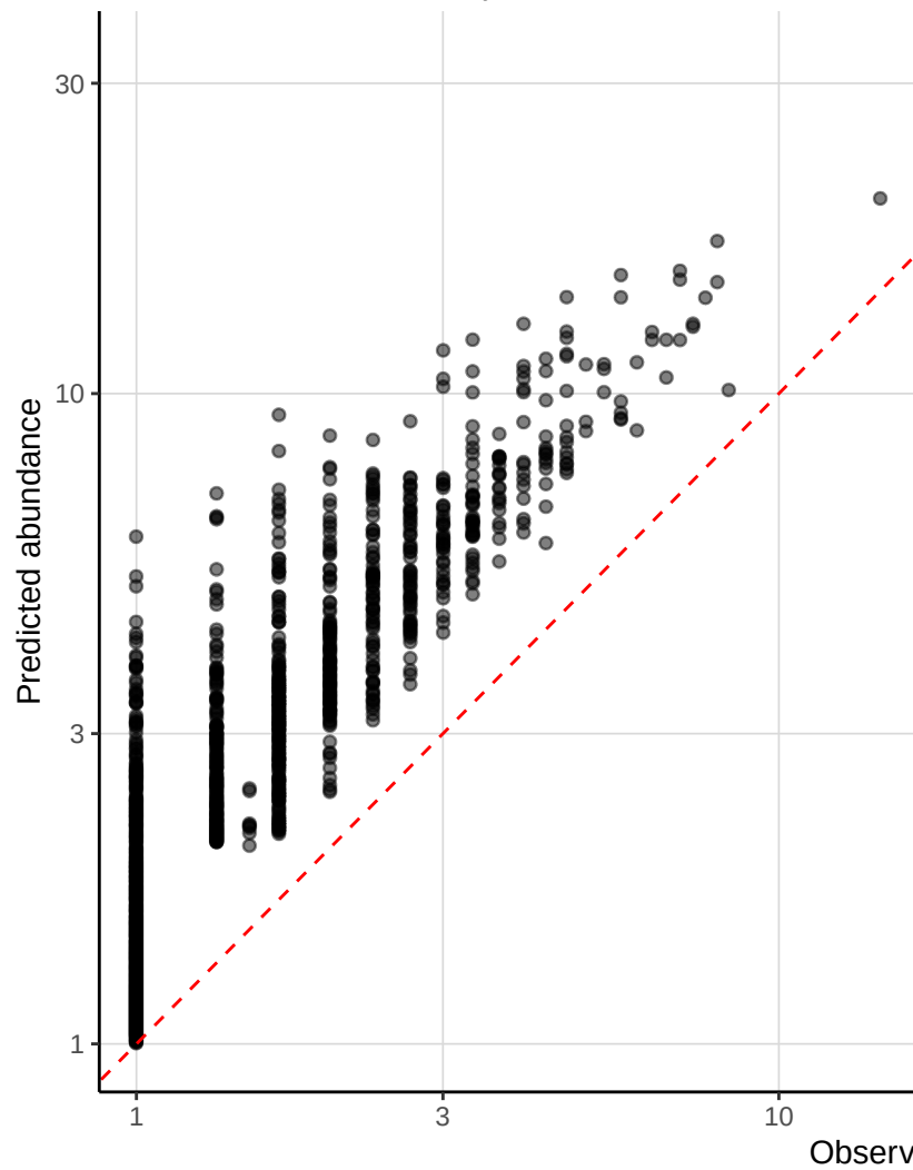
Bayesian
