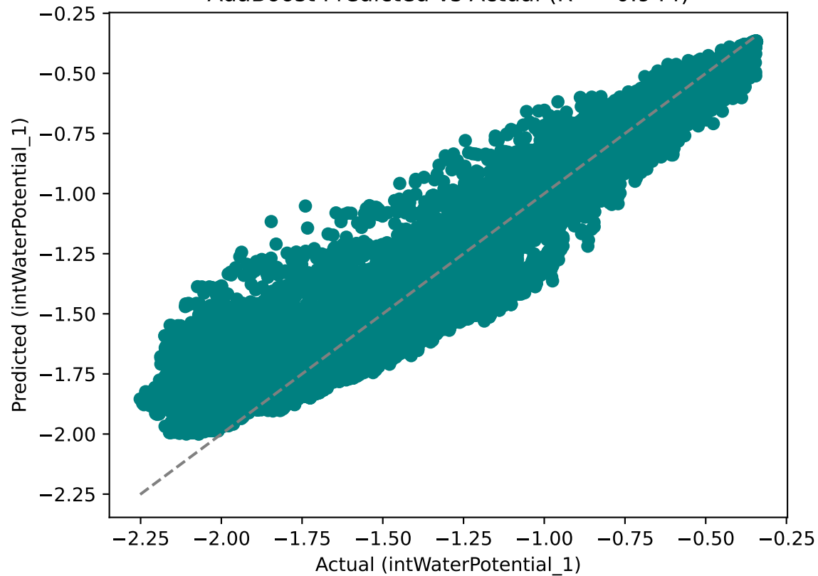
AdaBoost Predicted vs Actual ( R^2 = 0.944 )
