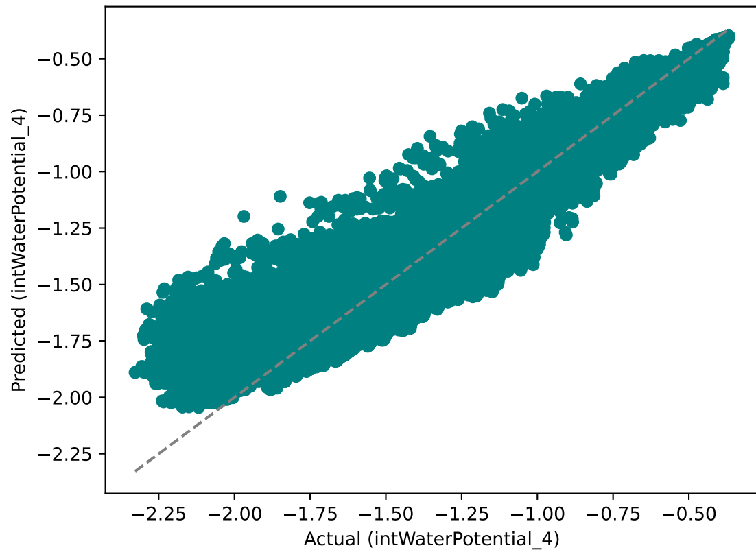
AdaBoost Predicted vs Actual ( R^2 = 0.935 )
