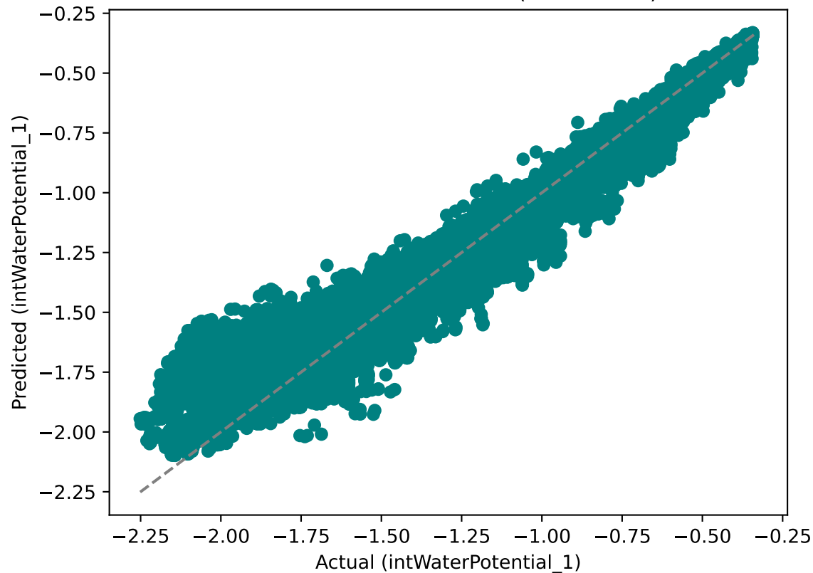
MLP Predicted vs Actual ( R^2 = 0.968 )
