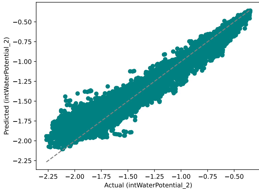
MLP Predicted vs Actual ( R^2 = 0.971 )
