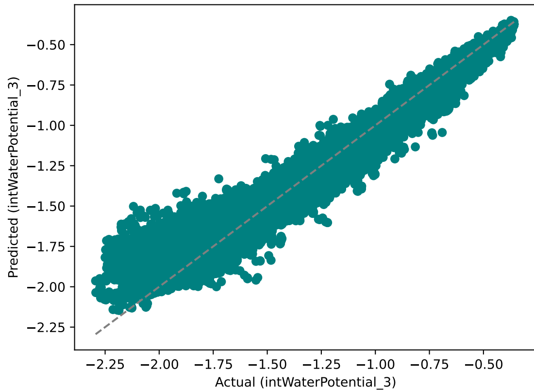
MLP Predicted vs Actual ( R^2 = 0.968 )
