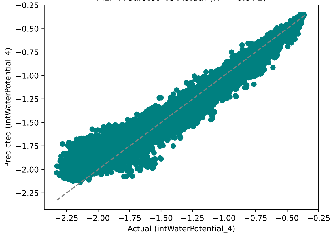
MLP Predicted vs Actual ( R^2 = 0.971 )
