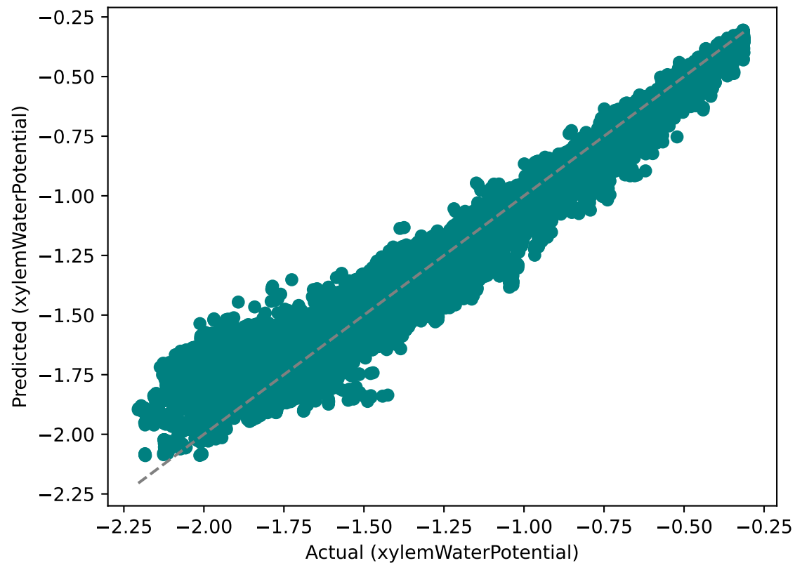
MLP Predicted vs Actual ( R^2 = 0.972 )
