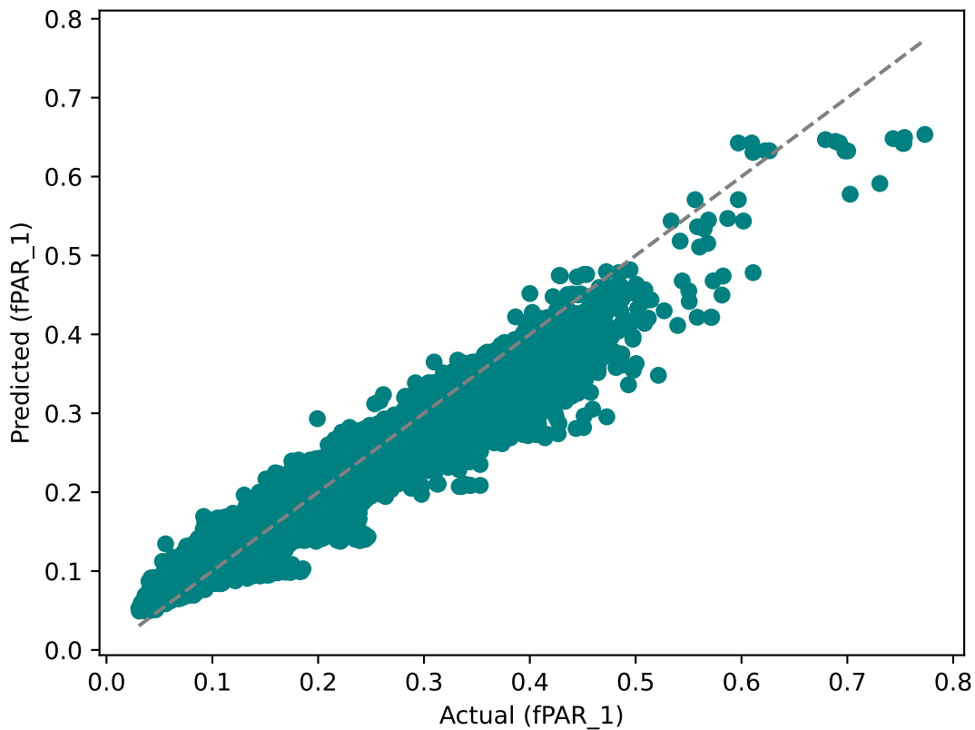
AdaBoost Predicted vs Actual ( R^2 = 0.926 )
