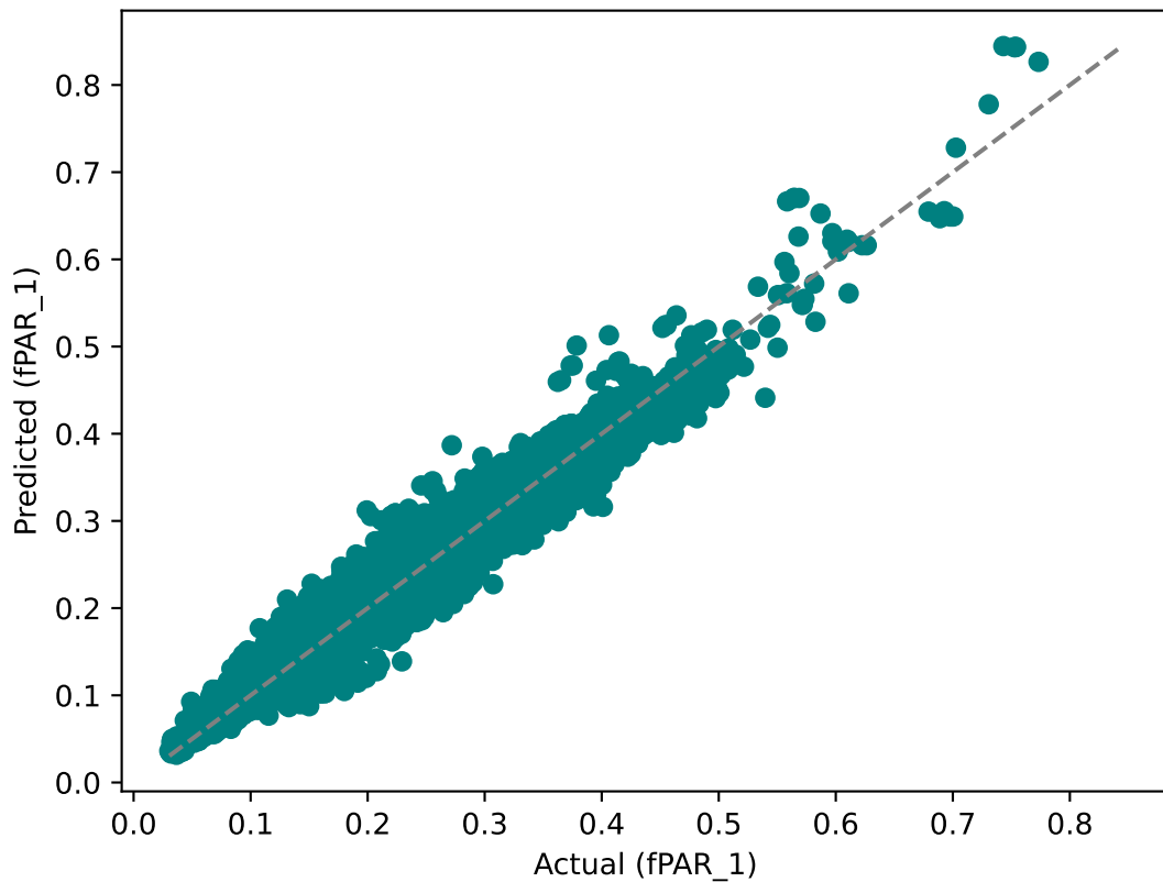
MLP Predicted vs Actual ( R^2 = 0.972 )
