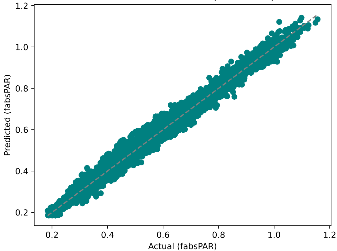
MLP Predicted vs Actual ( R^2 = 0.990 )
