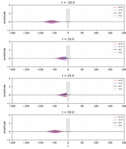
Figure 11. Blocked wave packet: E = 0.8 – 1.2 , centered at E_0 = 1.0 .
