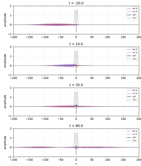
Figure 12. Partially blocked packet centered at the Part 3 second peak, E_0 = 1.32882395 .
