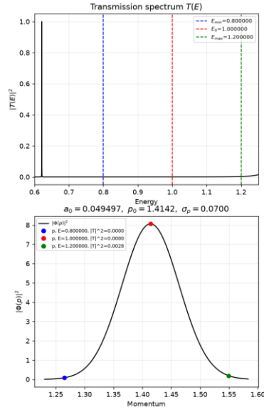
Figure 11. Blocked wave packet: E = 0.8 – 1.2 , centered at E_0 = 1.0 .
