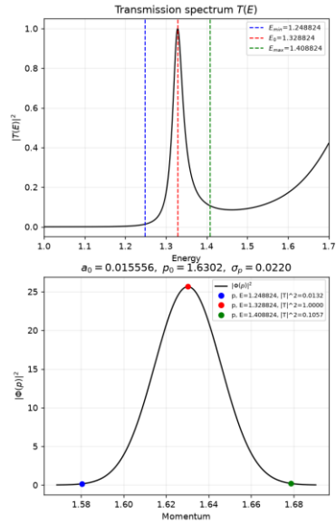
Figure 12. Partially blocked packet centered at the Part 3 second peak, E_0 = 1.32882395 .
