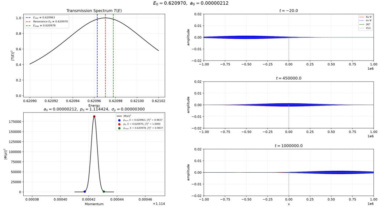
Figure 12. First-resonance packet centered at E_0=0.62097030 . The three full-range snapshots show the real and imaginary parts before, during and after transmission.
