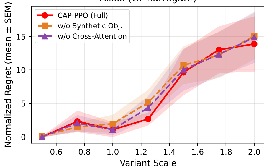
Alkox (GP surrogate)
