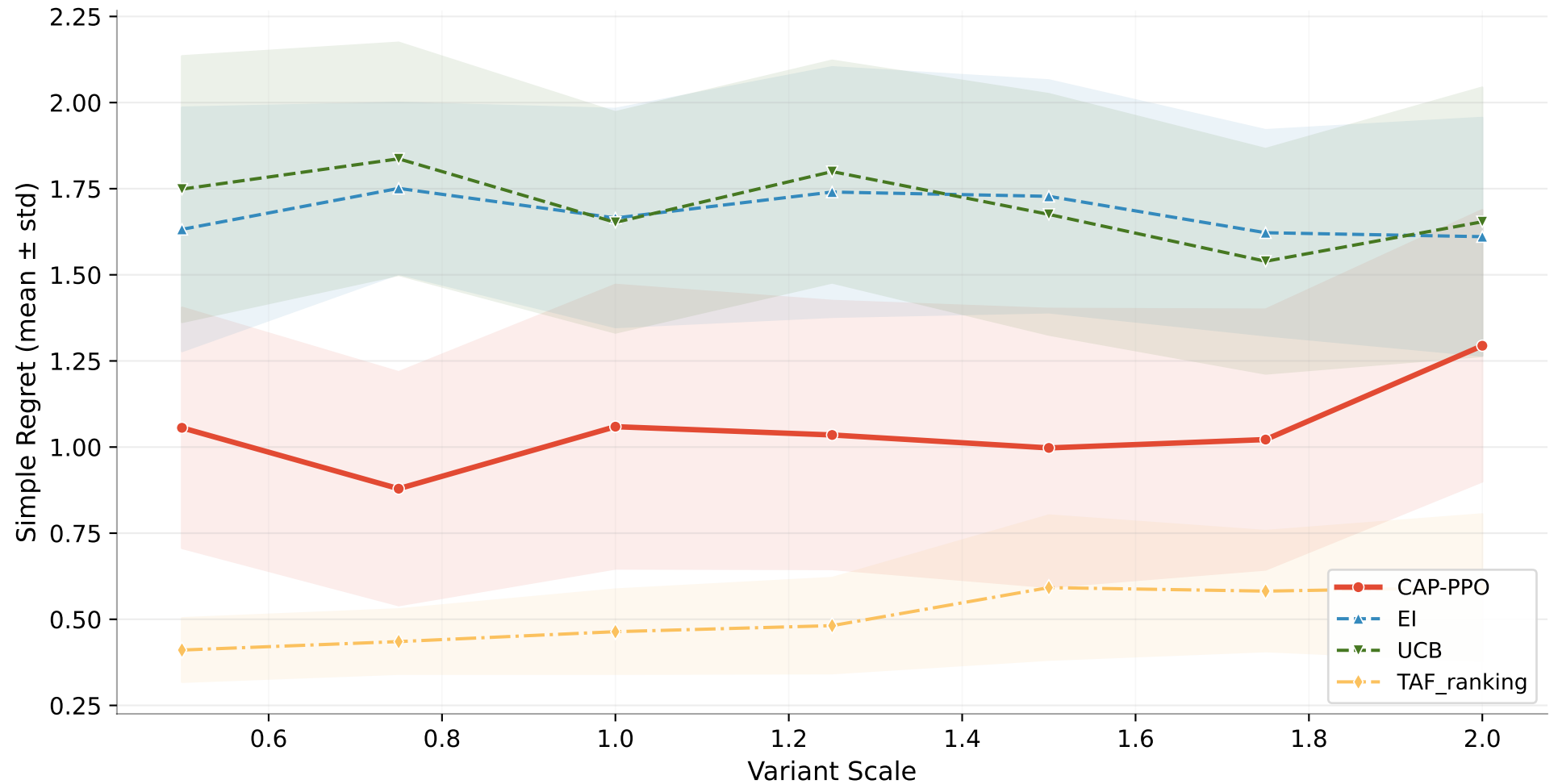
CAP-PPO vs Key Baselines — Hartmann 6D (GP surrogate)
