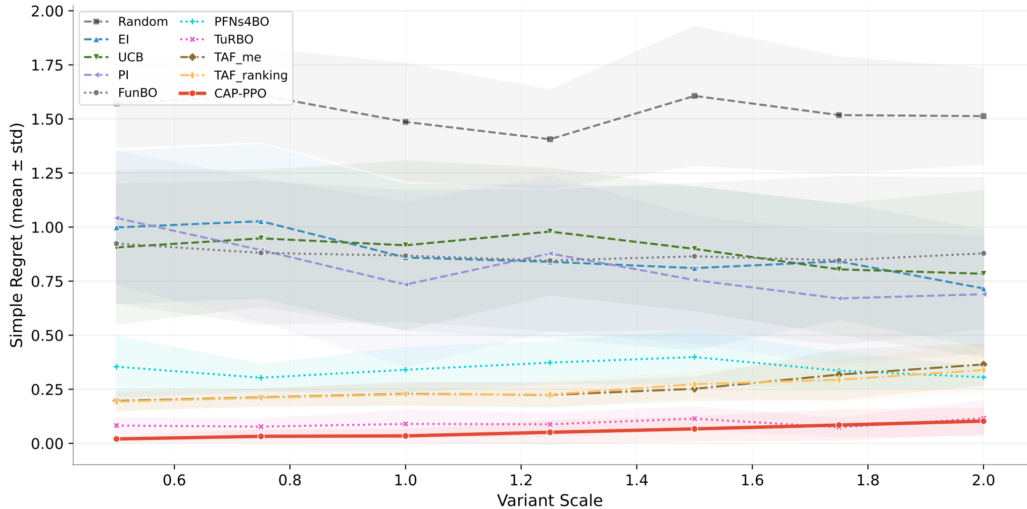
Hartmann 6D (GP surrogate)
