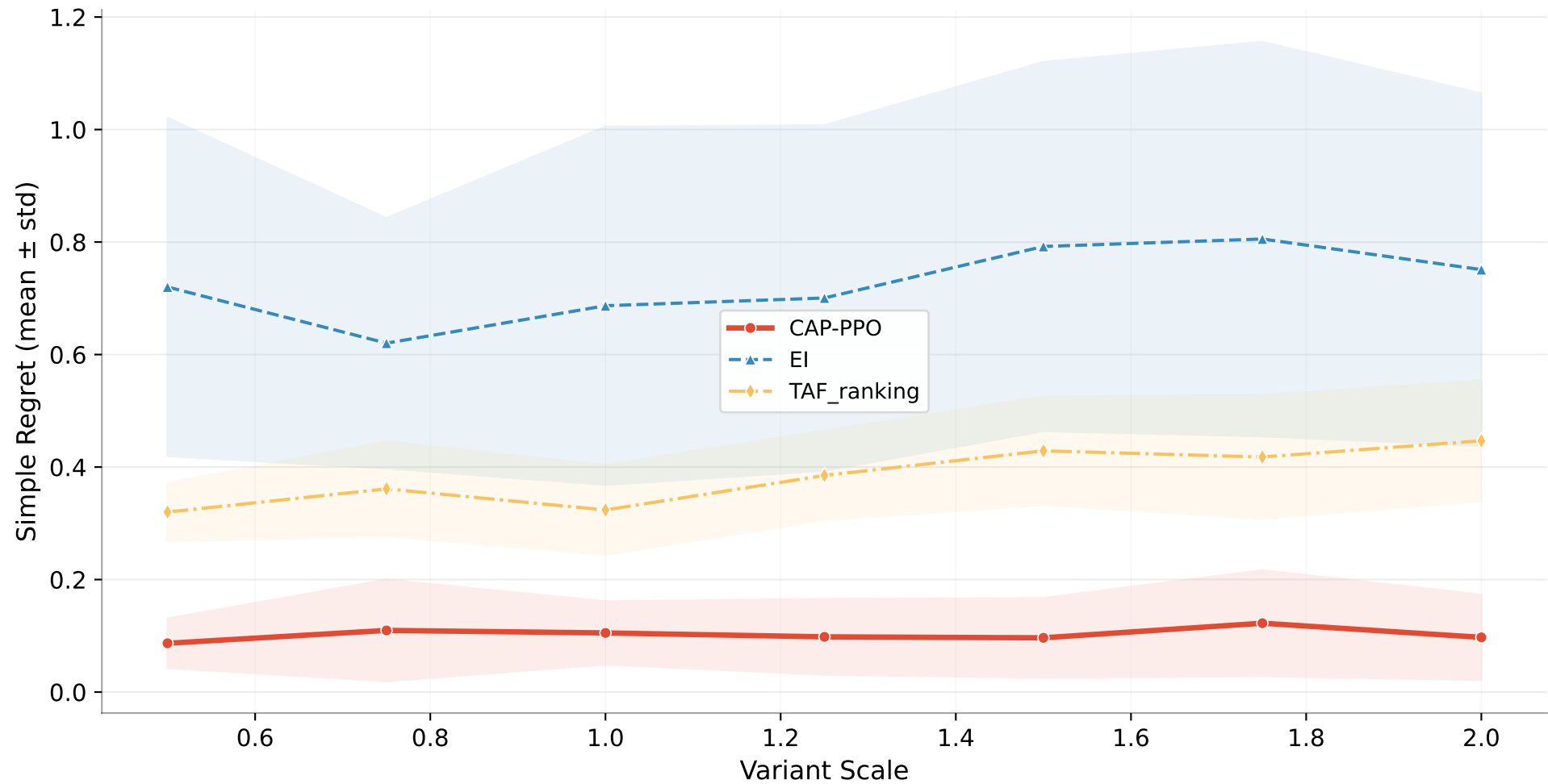
CAP-PPO vs Key Baselines — Hartmann 6D (TabPFN surrogate)
