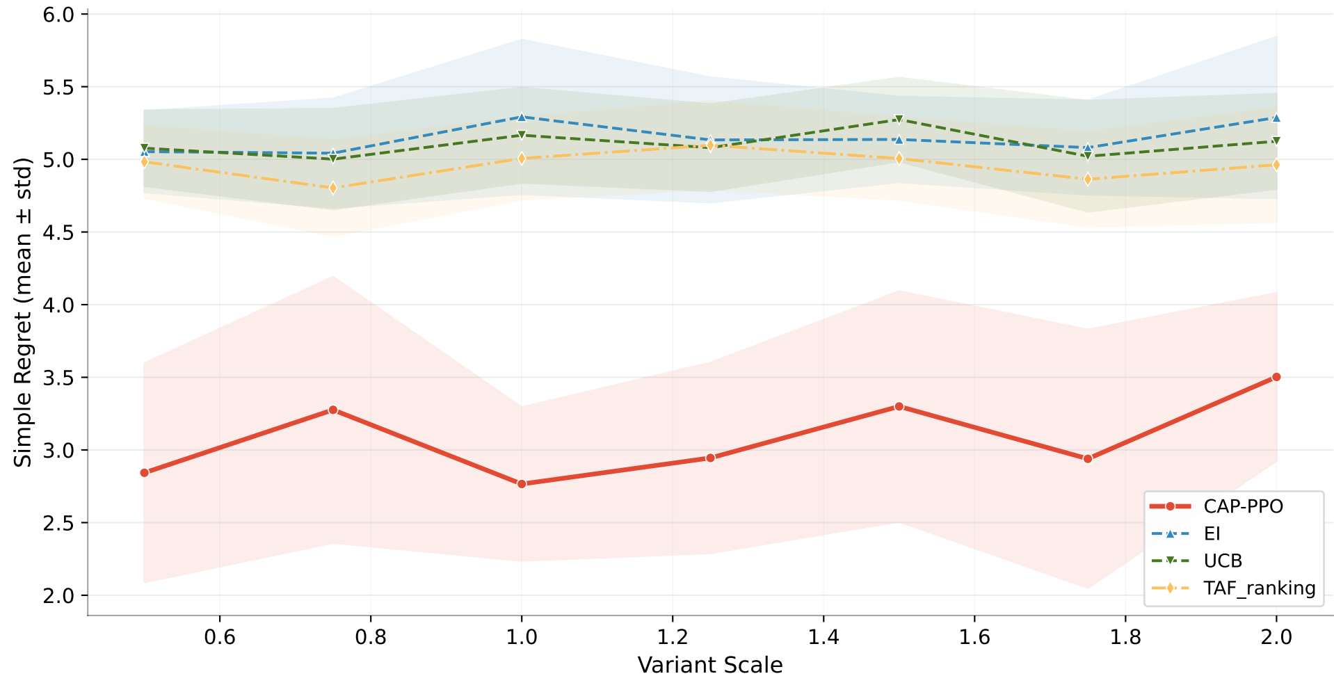
CAP-PPO vs Key Baselines — Ackley 10D (GP surrogate)
