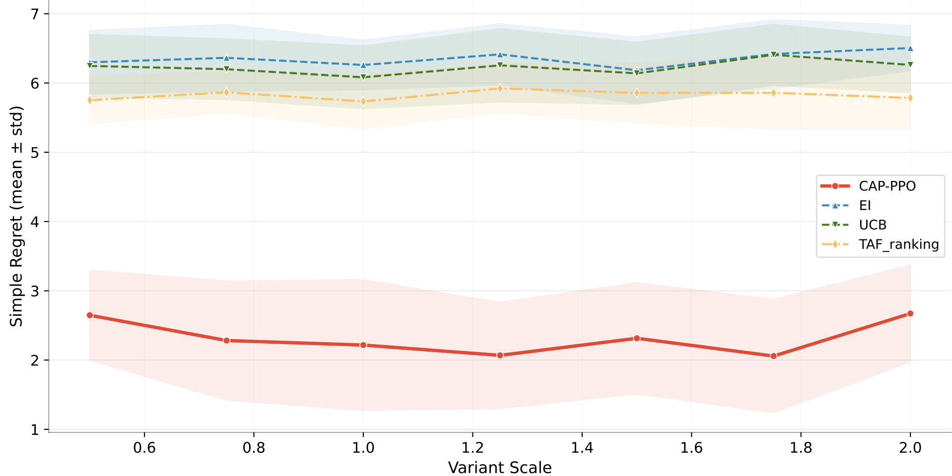
CAP-PPO vs Key Baselines — Ackley 10D (TabPFN surrogate)
