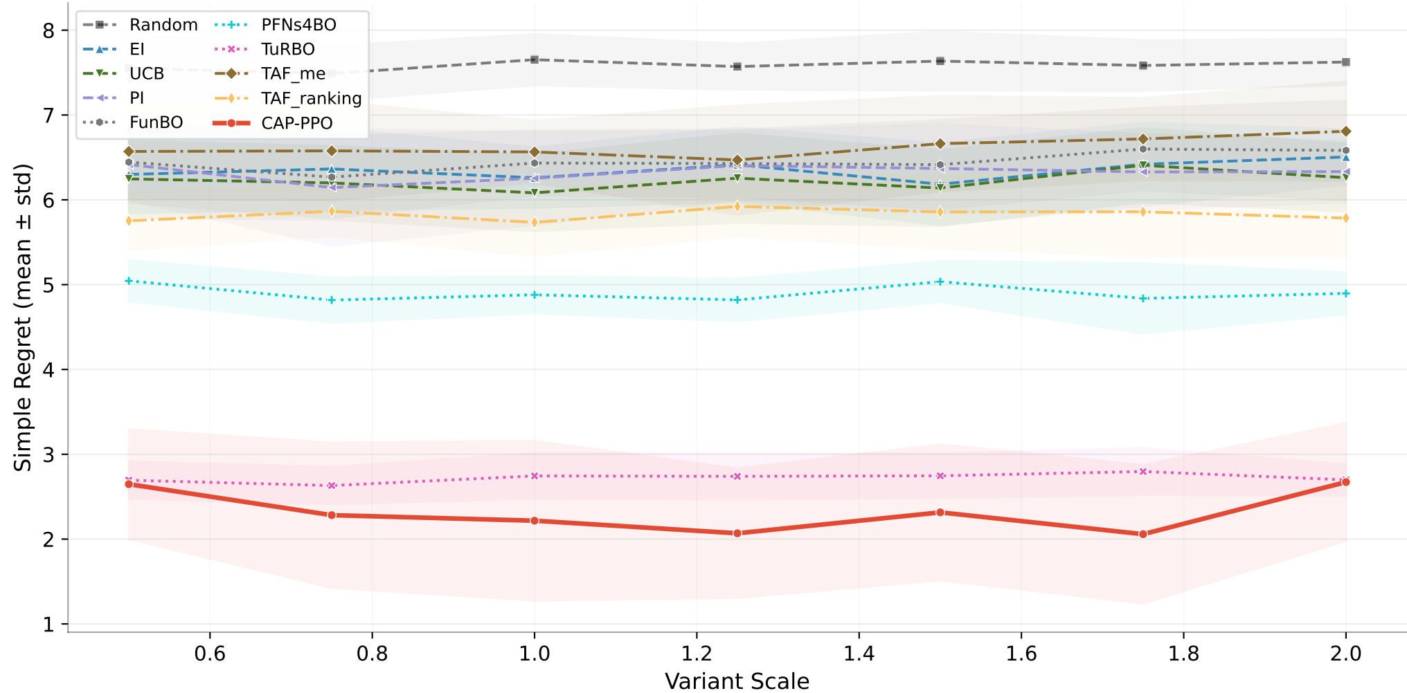
Ackley 10D (TabPFN surrogate)
