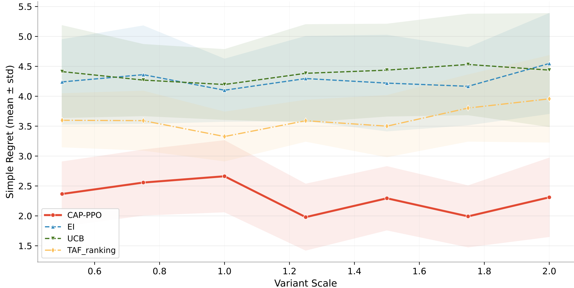
CAP-PPO vs Key Baselines — Ackley 5D (GP surrogate)
