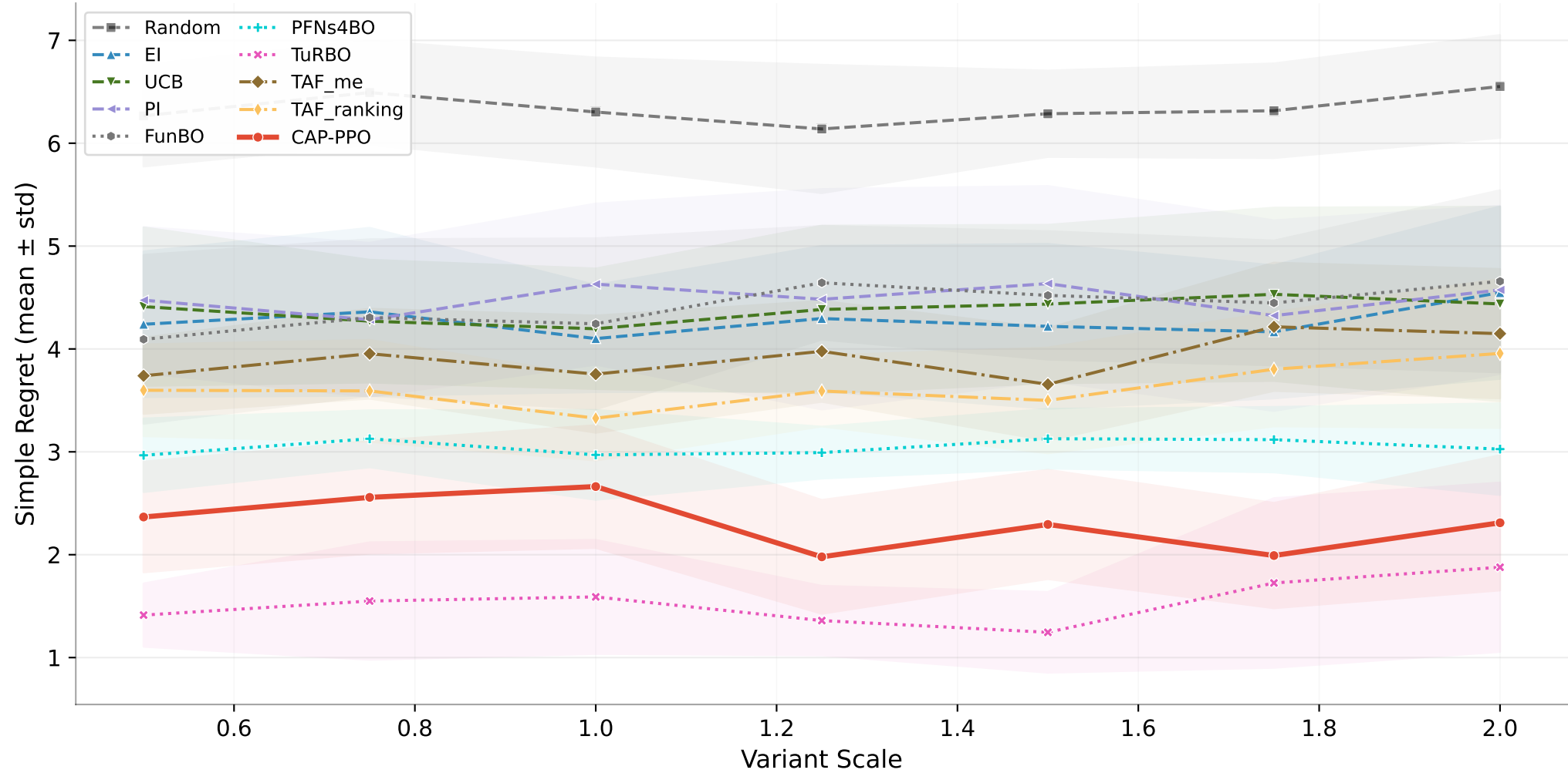
Ackley 5D (GP surrogate)
