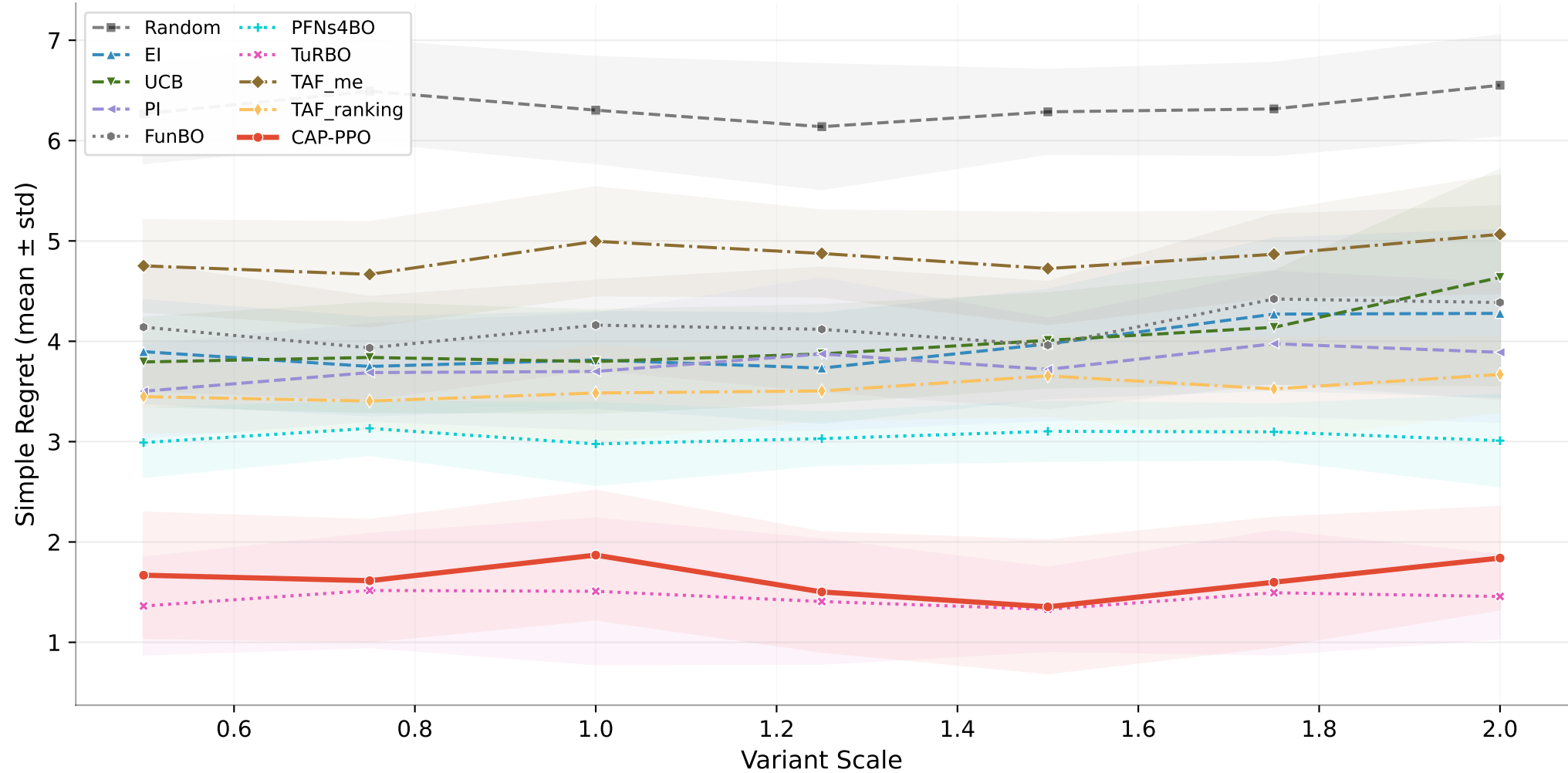
Ackley 5D (TabPFN surrogate)
