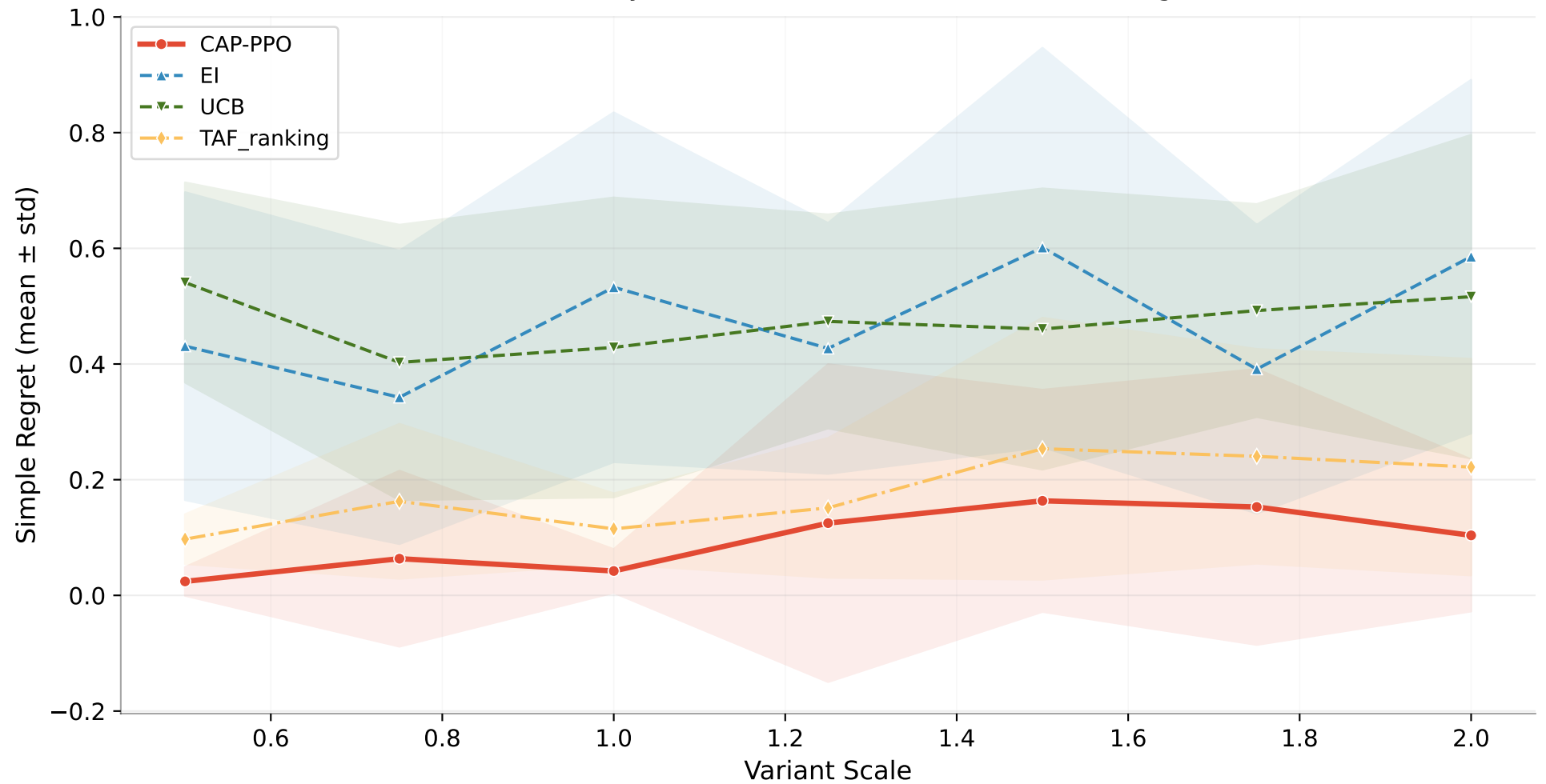
CAP-PPO vs Key Baselines — Hartmann 3D (GP surrogate)
