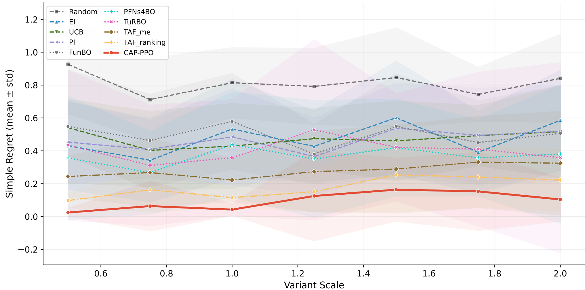
Hartmann 3D (GP surrogate)
