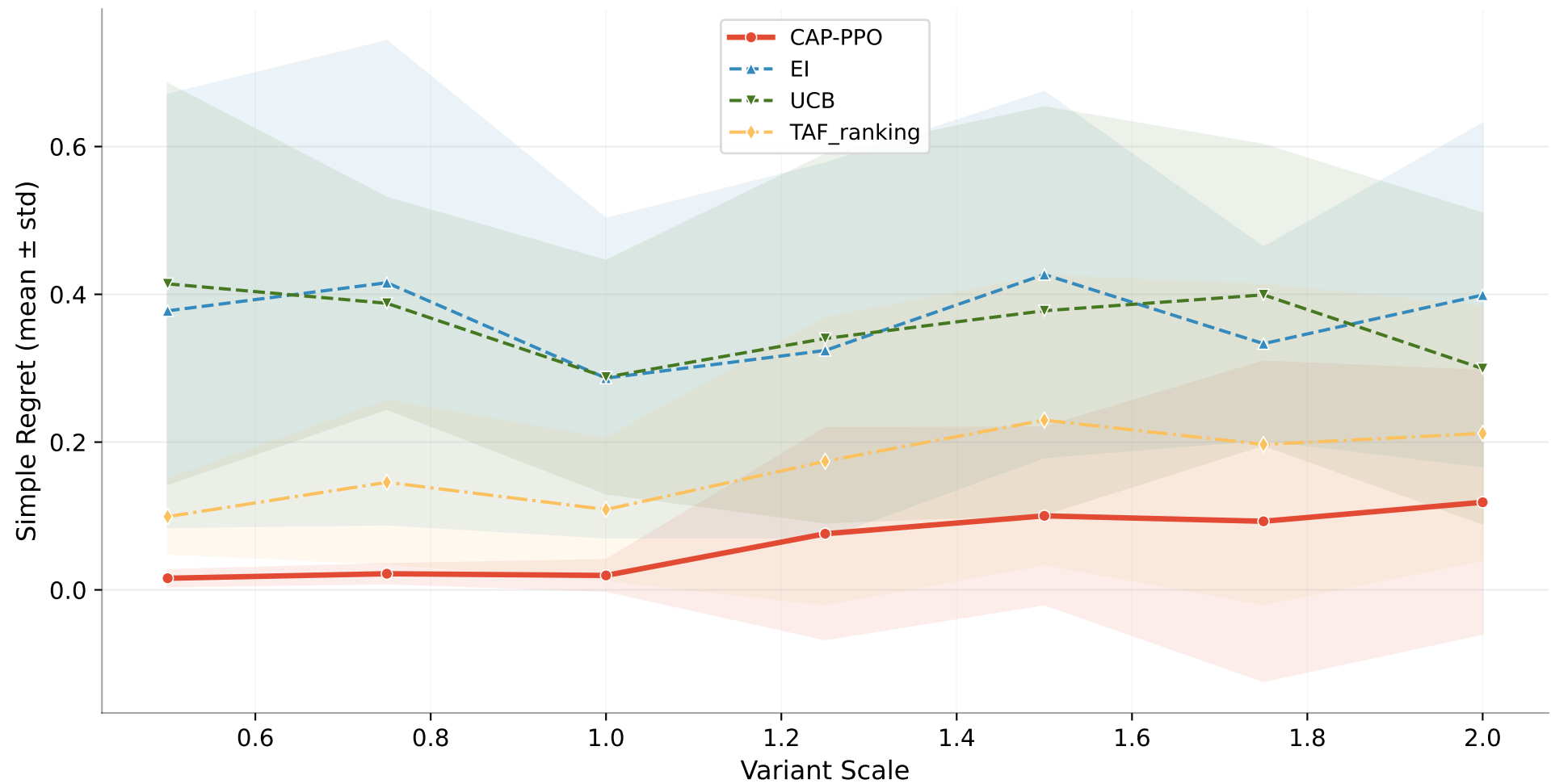
CAP-PPO vs Key Baselines — Hartmann 3D (TabPFN surrogate)
