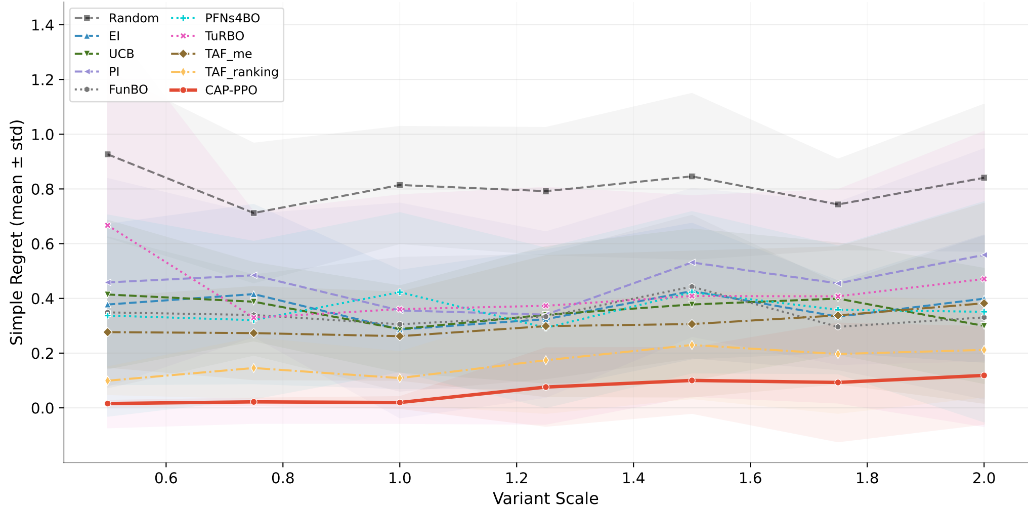
Hartmann 3D (TabPFN surrogate)
