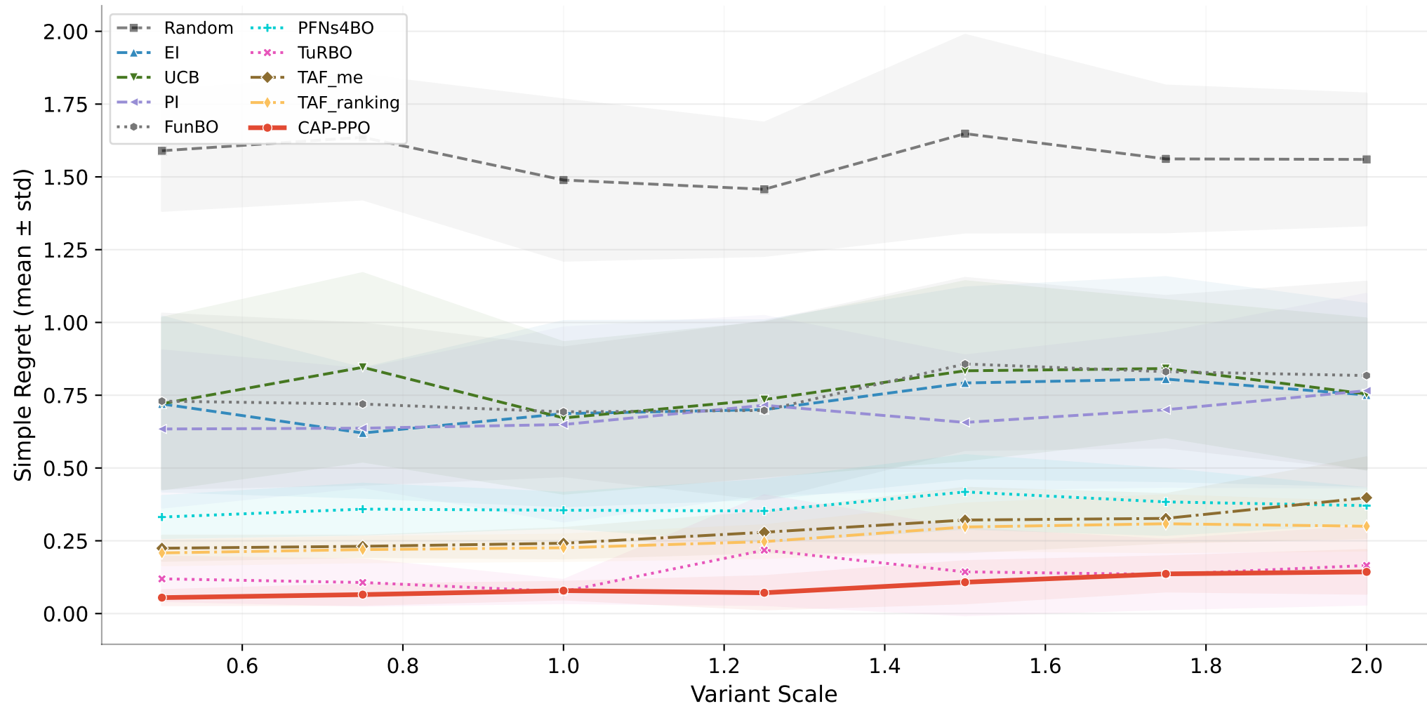
Hartmann 6D (TabPFN surrogate)
