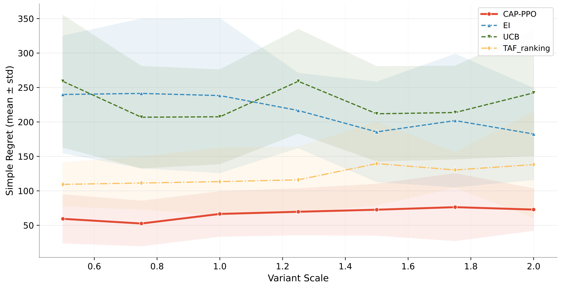
CAP-PPO vs Key Baselines — HPLC 6D (GP surrogate)
