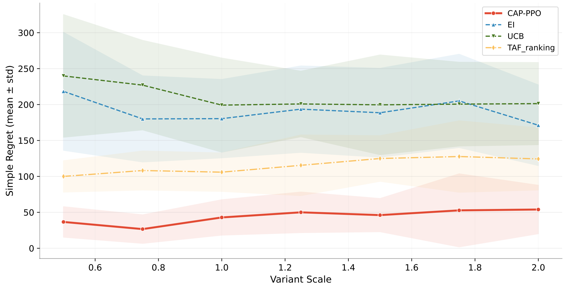
CAP-PPO vs Key Baselines — HPLC 6D (TabPFN surrogate)
